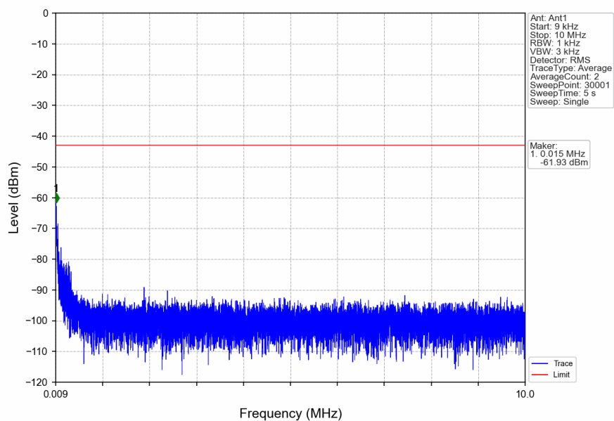
n41_30kHz_SISO_NTNV_100MHz_DFT-s-OFDM_PI/2_BPSK_2592.99MHz_Edge_1RB_Left
