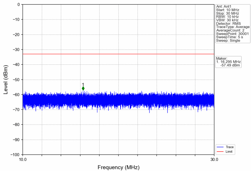
n41_30kHz_SISO_NTNV_90MHz_CP-OFDM_QPSK_2592.99MHz_Edge_1RB_Left
