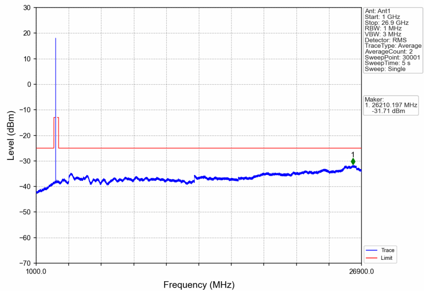
n41_30kHz_SISO_NTNV_90MHz_CP-OFDM_QPSK_2592.99MHz_Edge_1RB_Left
