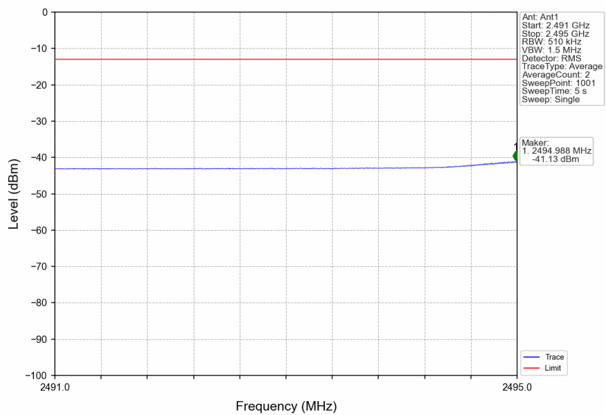
n41_30kHz_SISO_NTNV_100MHz_DFT-s-OFDM_QPSK_2546.01MHz_Edge_1RB_Left
