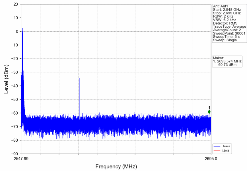
n41_30kHz_SISO_NTNV_90MHz_CP-OFDM_QPSK_2592.99MHz_Edge_1RB_Left
