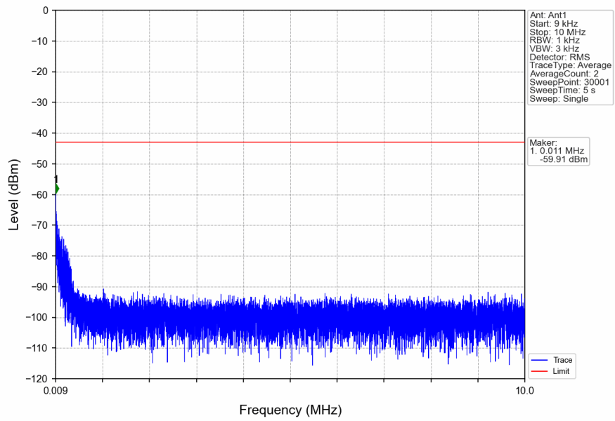
n41_30kHz_SISO_NTNV_90MHz_CP-OFDM_QPSK_2592.99MHz_Edge_1RB_Left
