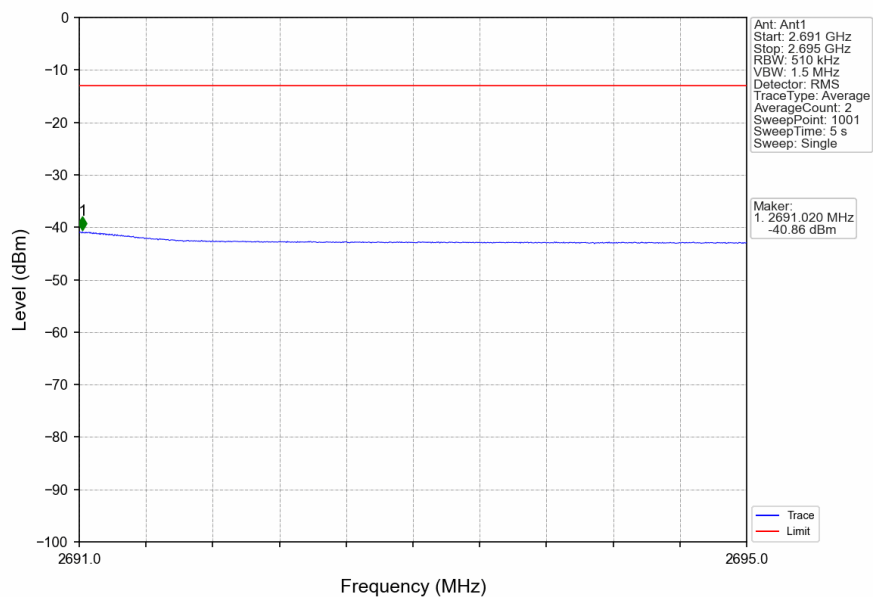
n41_30kHz_SISO_NTNV_90MHz_CP-OFDM_QPSK_2644.98MHz_Edge_1RB_Right
