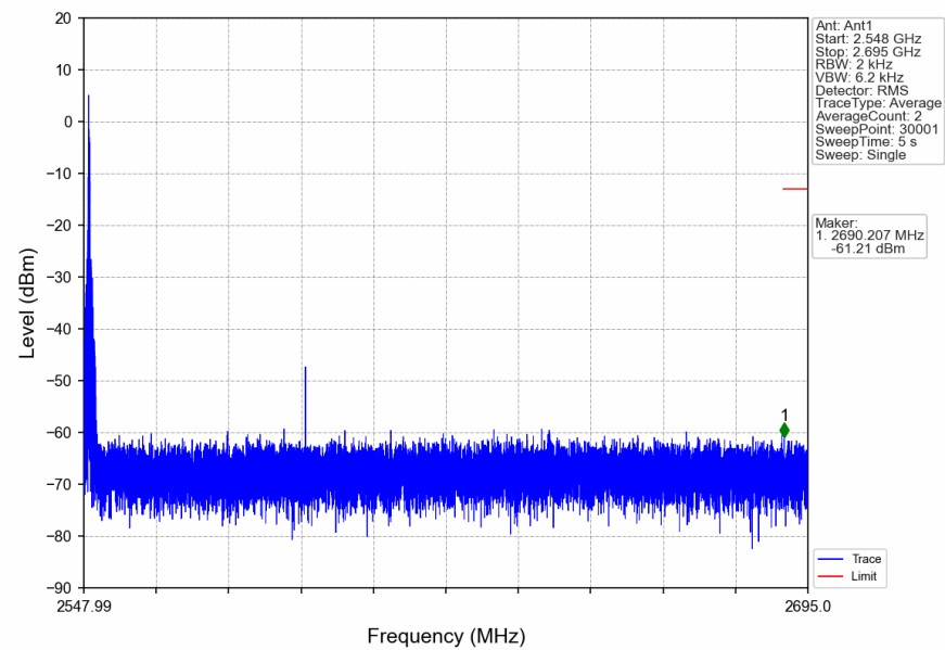
n41_30kHz_SISO_NTNV_90MHz_DFT-s-OFDM_QPSK_2592.99MHz_Edge_1RB_Left
