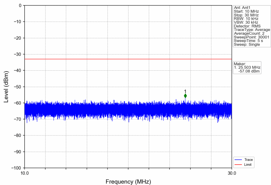
n41_30kHz_SISO_NTNV_100MHz_DFT-s-OFDM_PI/2_BPSK_2592.99MHz_Edge_1RB_Left
