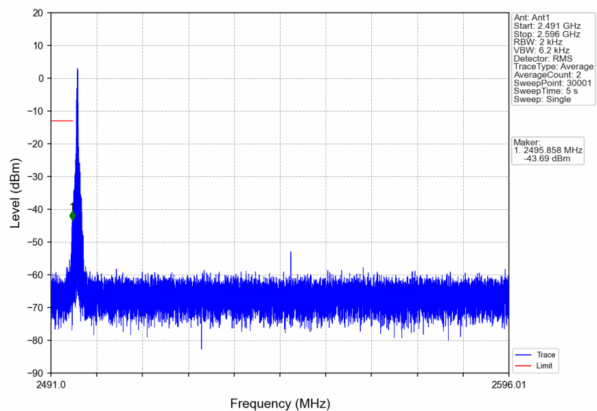
n41_30kHz_SISO_NTNV_100MHz_DFT-s-OFDM_QPSK_2546.01MHz_Edge_1RB_Left
