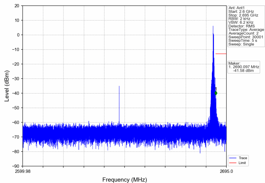
n41_30kHz_SISO_NTNV_90MHz_CP-OFDM_QPSK_2644.98MHz_Edge_1RB_Right
