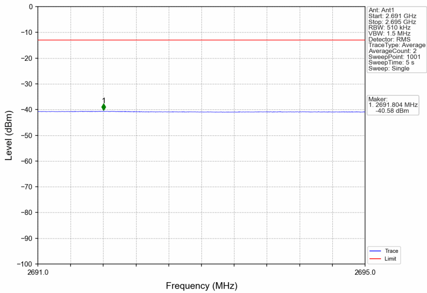
n41_30kHz_SISO_NTNV_90MHz_DFT-s-OFDM_QPSK_2644.98MHz_Outer_Full
