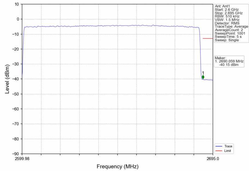
n41_30kHz_SISO_NTNV_90MHz_DFT-s-OFDM_QPSK_2644.98MHz_Outer_Full
