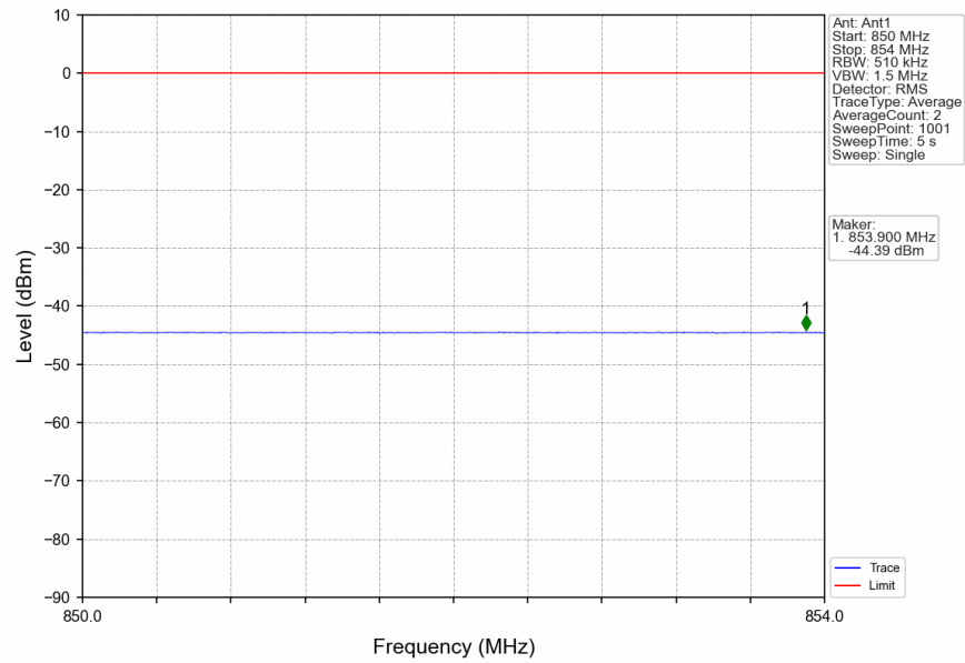
n5_15kHz_SISO_NTNV_5MHz_DFT-s-OFDM_QPSK_836.5MHz_Edge_1RB_Left
