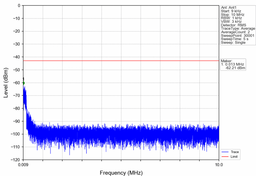
n5_15kHz_SISO_NTNV_5MHz_DFT-s-OFDM QPSK_846.5MHz_Inner_1RB_Right
