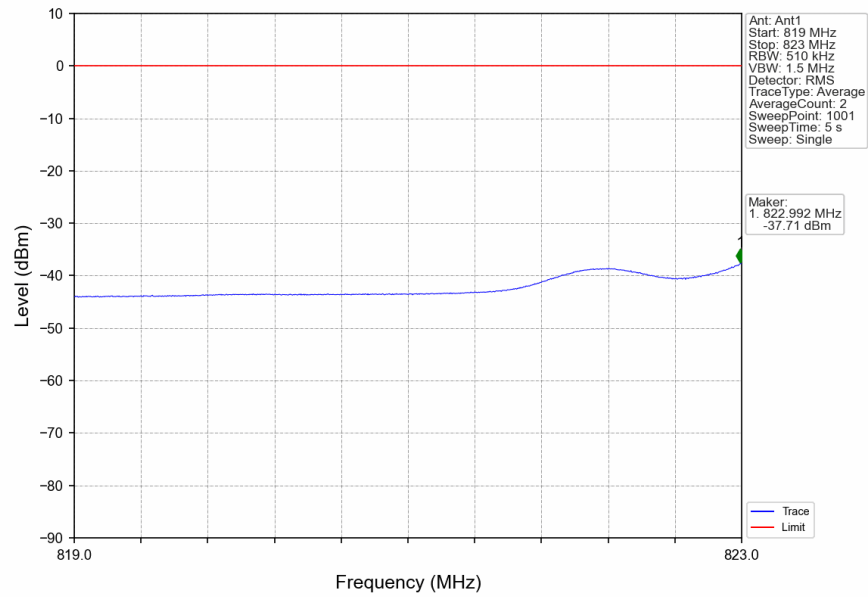
n5_15kHz_SISO_NTNV_5MHz_DFT-s-OFDM_QPSK_826.5MHz_Edge_1RB_Left
