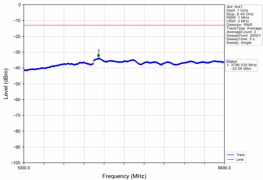
n5_15kHz_SISO_NTNV_5MHz_CP-OFDM QPSK_826.5MHz_Inner_1RB_Left
