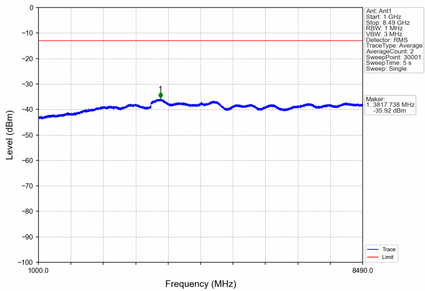
n5_15kHz_SISO_NTNV_5MHz_CP-OFDM_QPSK_836.5MHz_Edge_1RB_Left
