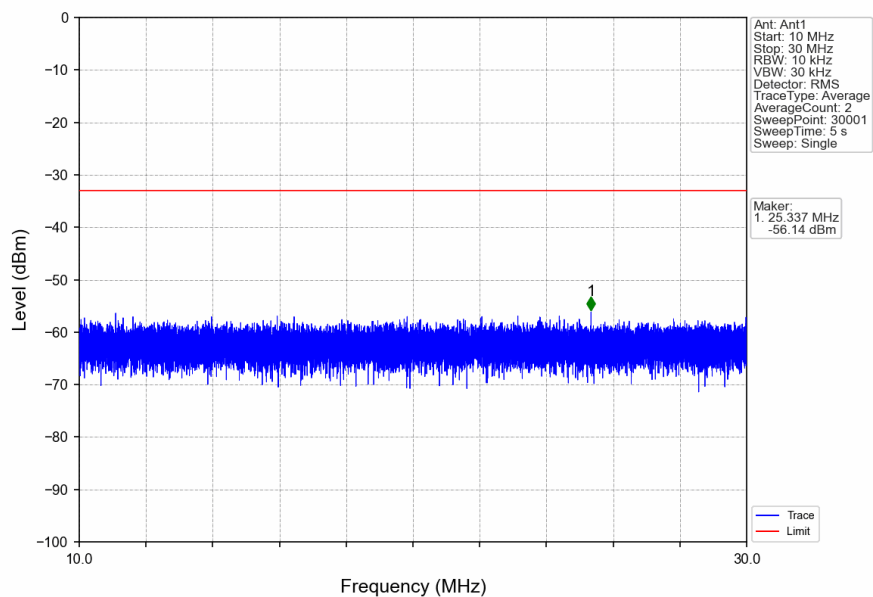
n5_15kHz_SISO_NTNV_5MHz_DFT-s-OFDM QPSK_846.5MHz_Inner_1RB_Right
