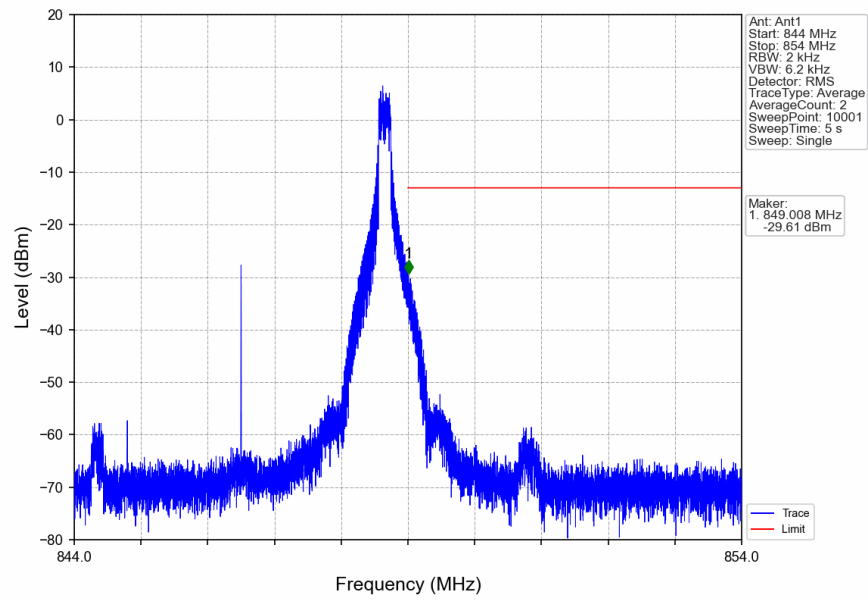
n5_15kHz_SISO_NTNV_5MHz_DFT-s-OFDM QPSK_846.5MHz_Edge_1RB_Right
