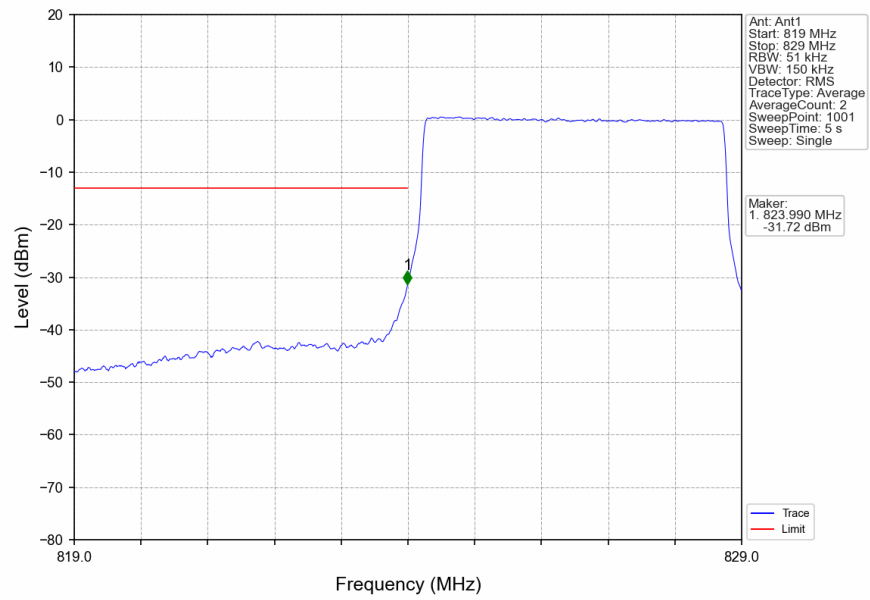
n5_15kHz_SISO_NTNV_5MHz_CP-OFDM_QPSK_826.5MHz_Outer_Full
