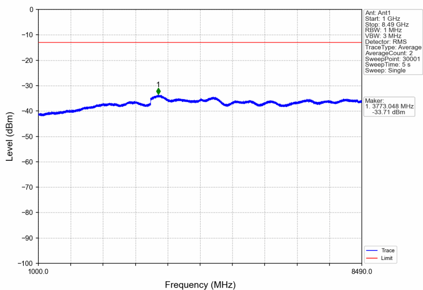
n5_15kHz_SISO_NTNV_5MHz_DFT-s-OFDM PI/2 BPSK_836.5MHz_Edge_1RB_Left
