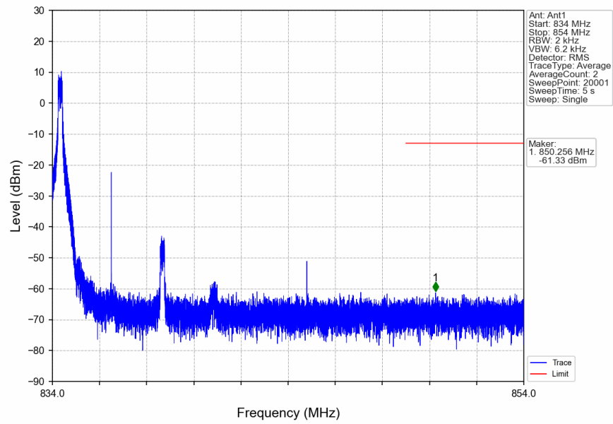
n5_15kHz_SISO_NTNV_5MHz_DFT-s-OFDM_QPSK_836.5MHz_Edge_1RB_Left
