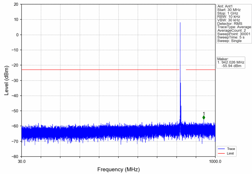
n5_15kHz_SISO_NTNV_5MHz_CP-OFDM_QPSK_826.5MHz_Edge_1RB_Left
