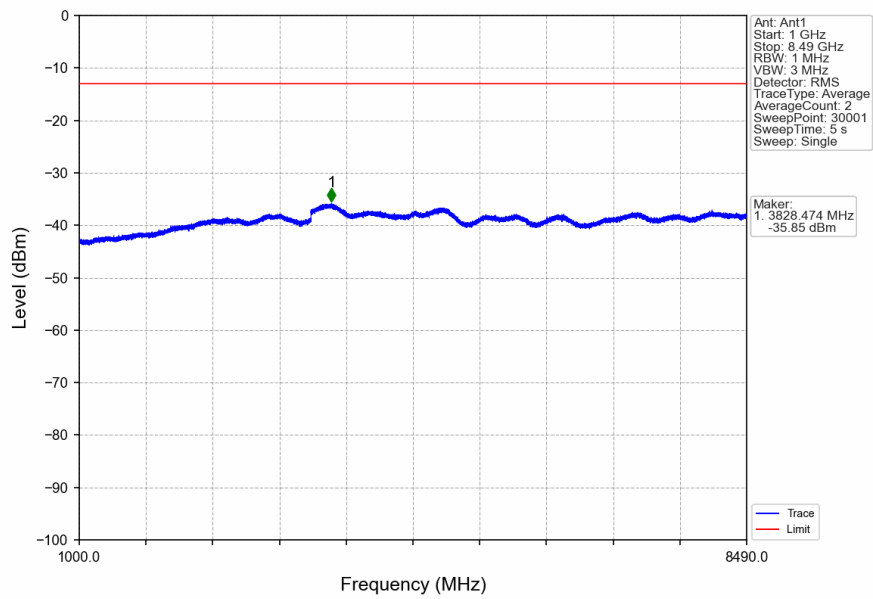
n5_15kHz_SISO_NTNV_5MHz_CP-OFDM_QPSK_826.5MHz_Edge_1RB_Left
