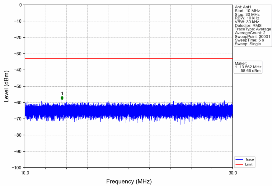
n5_15kHz_SISO_NTNV_5MHz_DFT-s-OFDM_QPSK_846.5MHz_Edge_1RB_Right
