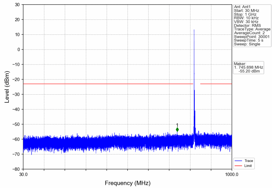
n5_15kHz_SISO_NTNV_5MHz_CP-OFDM QPSK_826.5MHz_Inner_1RB_Left
