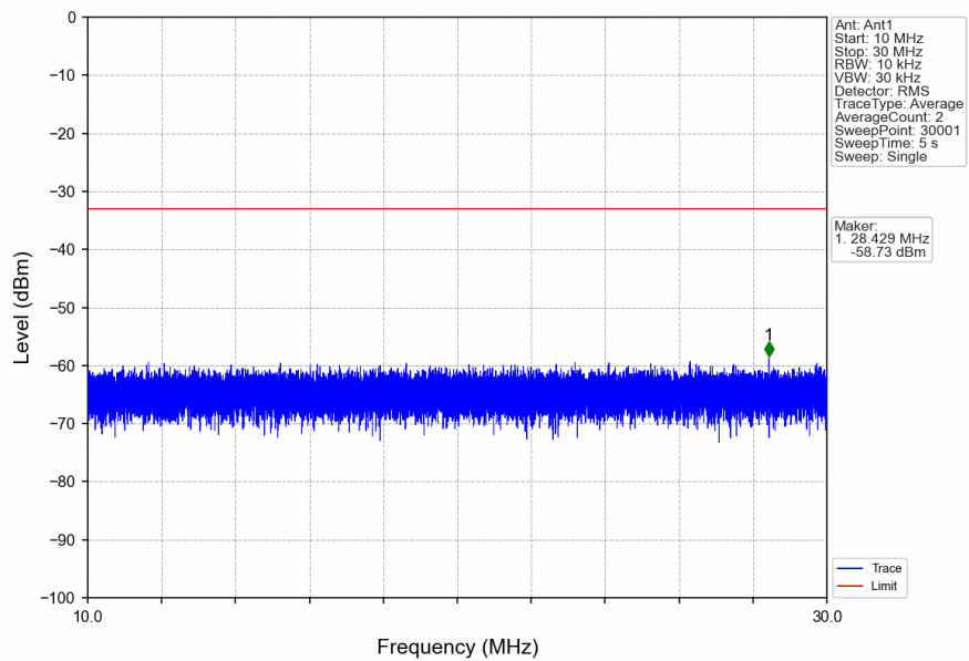
n5_15kHz_SISO_NTNV_5MHz_DFT-s-OFDM_QPSK_826.5MHz_Edge_1RB_Left
