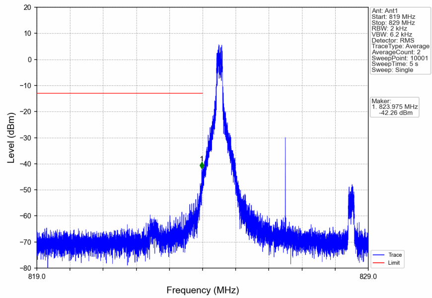
n5_15kHz_SISO_NTNV_5MHz_DFT-s-OFDM_QPSK_826.5MHz_Inner_1RB_Left
