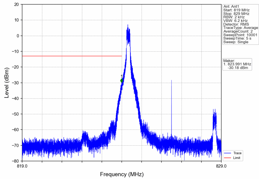
n5_15kHz_SISO_NTNV_5MHz_DFT-s-OFDM_QPSK_826.5MHz_Edge_1RB_Left
