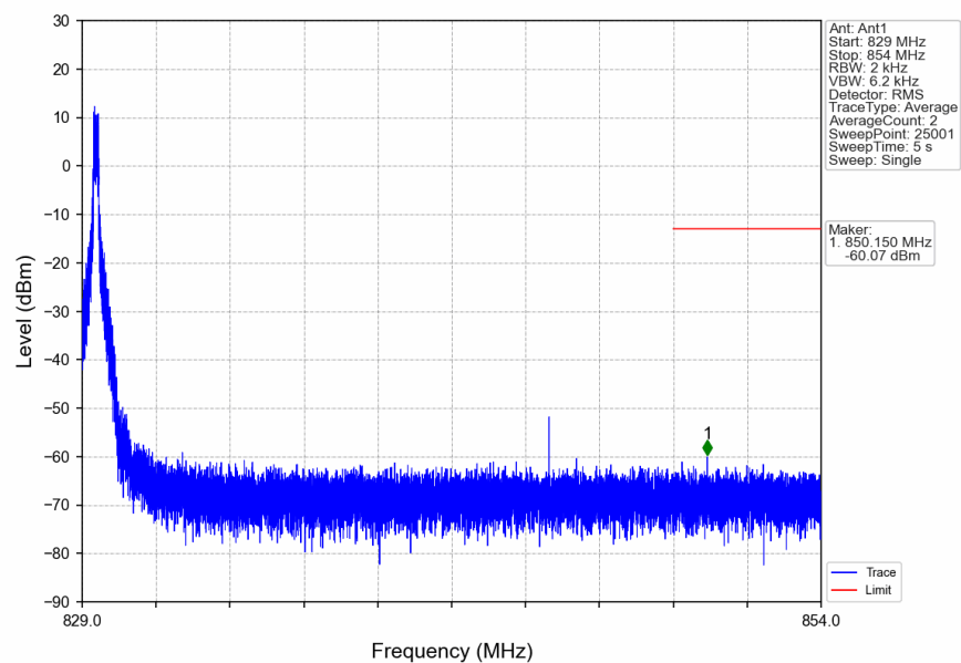
n5_15kHz_SISO_NTNV_15MHz_DFT-s-OFDM_PI/2_BPSK_836.5MHz_Edge_1RB_Left
