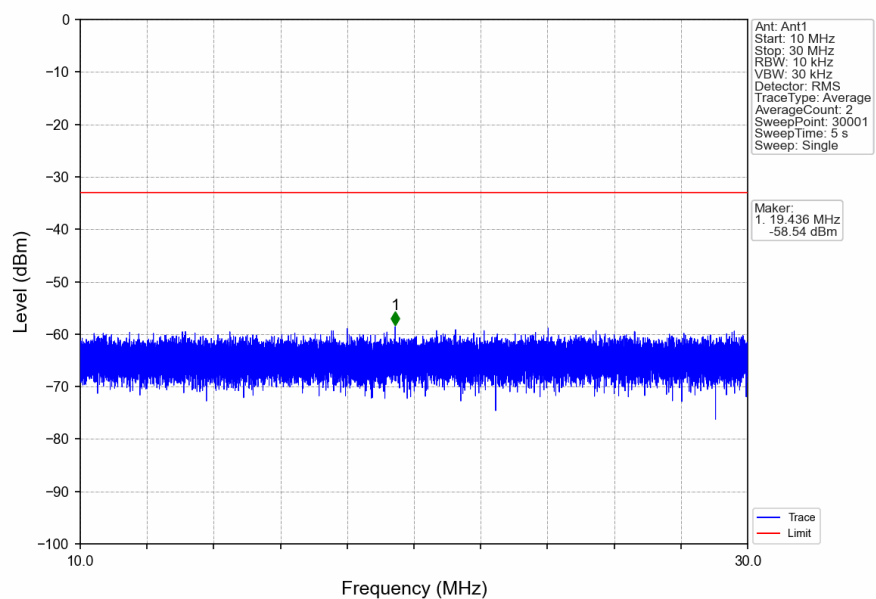
n5_15kHz_SISO_NTNV_15MHz_DFT-s-OFDM QPSK_831.5MHz_Edge_1RB_Left
