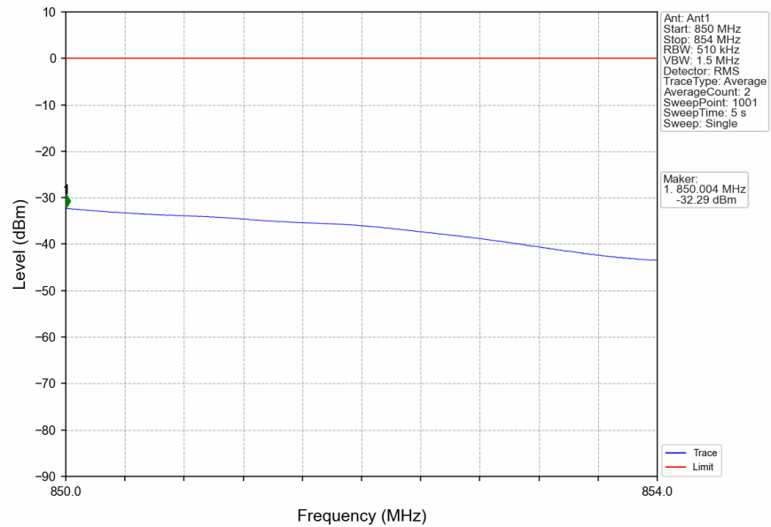
n5_15kHz_SISO_NTNV_10MHz_CP-OFDM_QPSK_844MHz_Outer_Full
