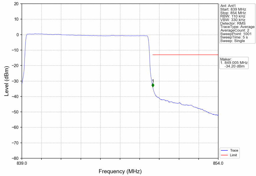
n5_15kHz_SISO_NTNV_10MHz_CP-OFDM_QPSK_844MHz_Outer_Full
