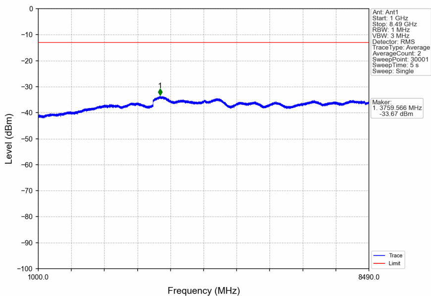
n5_15kHz_SISO_NTNV_15MHz_DFT-s-OFDM_PI/2_BPSK_831.5MHz_Edge_1RB_Left
