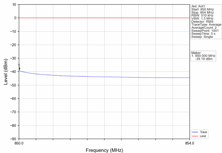
n5_15kHz_SISO_NTNV_15MHz_DFT-s-OFDM PI/2 BPSK_841.5MHz_Edge_1RB_Right
