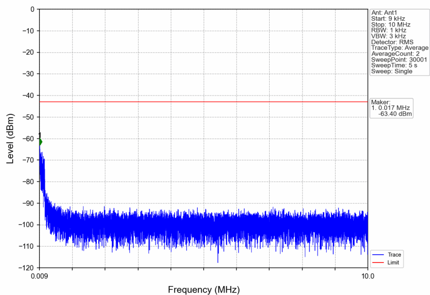
n5_15kHz_SISO_NTNV_15MHz_DFT-s-OFDM_QPSK_841.5MHz_Edge_1RB_Right
