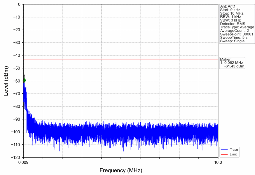
n5_15kHz_SISO_NTNV_15MHz_DFT-s-OFDM_QPSK_841.5MHz_Inner_1RB_Right
