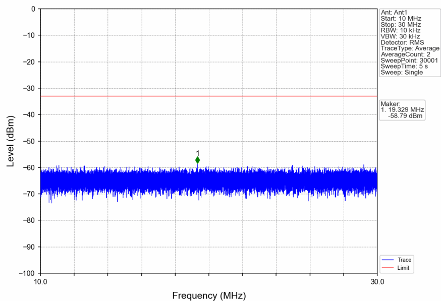
n5_15kHz_SISO_NTNV_15MHz_DFT-s-OFDM_QPSK_841.5MHz_Edge_1RB_Right
