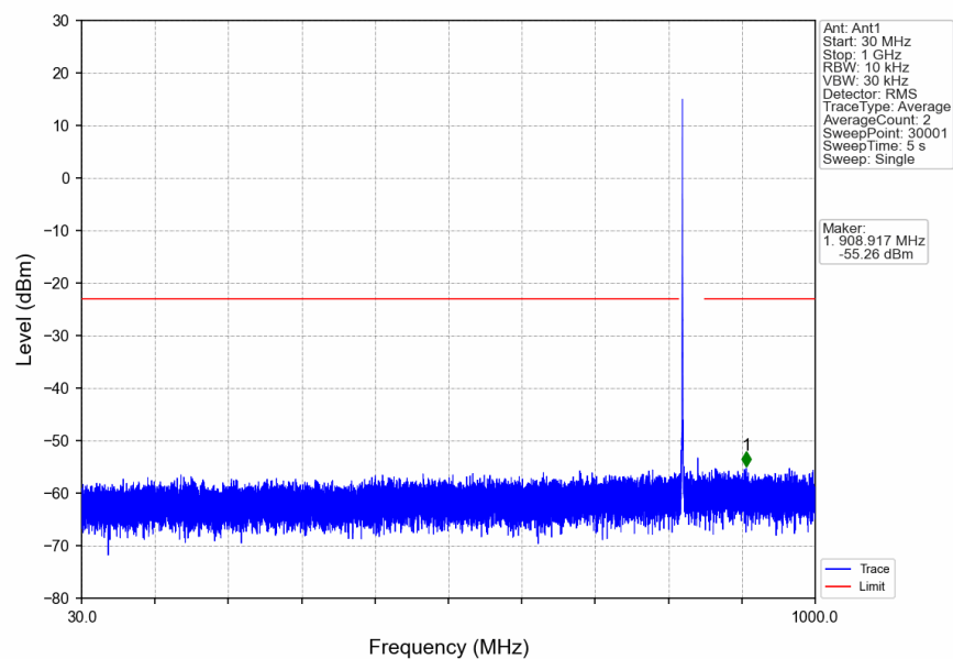
n5_15kHz_SISO_NTNV_15MHz_DFT-s-OFDM_PI/2_BPSK_831.5MHz_Edge_1RB_Left
