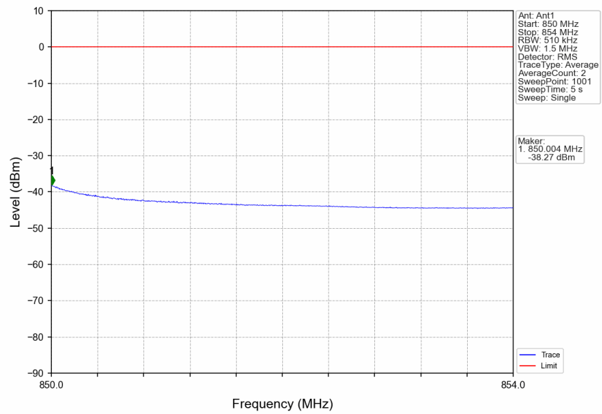
n5_15kHz_SISO_NTNV_15MHz_DFT-s-OFDM_QPSK_841.5MHz_Edge_1RB_Right
