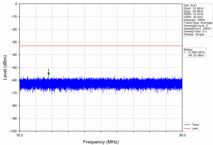
n5_15kHz_SISO_NTNV_15MHz_DFT-s-OFDM_QPSK_841.5MHz_Inner_1RB_Right
