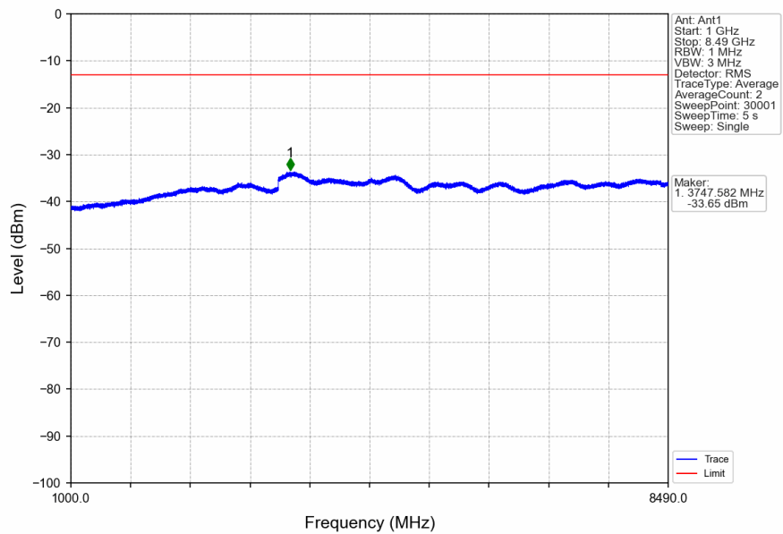
n5_15kHz_SISO_NTNV_15MHz_DFT-s-OFDM PI/2 BPSK_836.5MHz_Edge_1RB_Left
