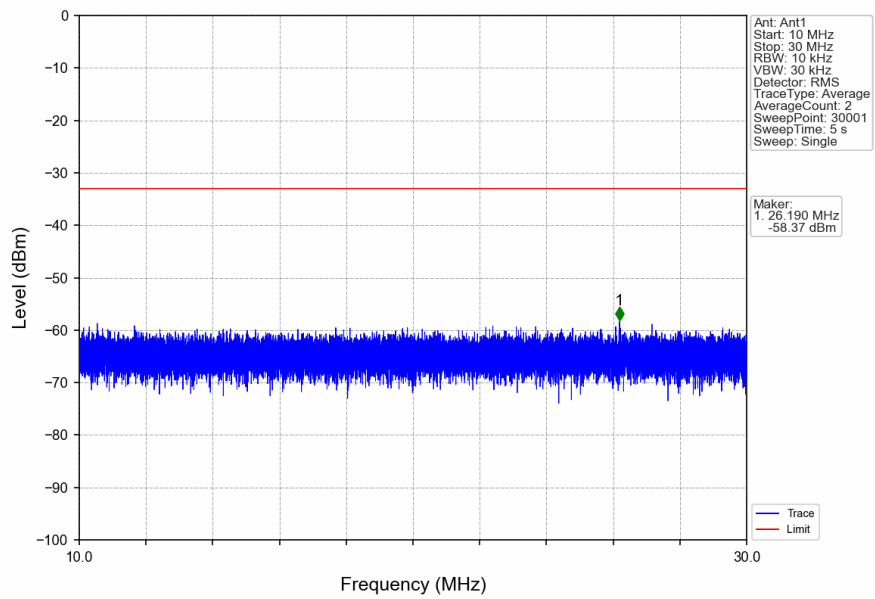
n5_15kHz_SISO_NTNV_15MHz_CP-OFDM_QPSK_841.5MHz_Edge_1RB_Right
