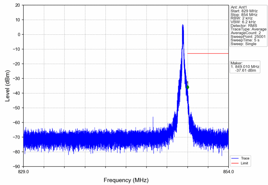
n5_15kHz_SISO_NTNV_20MHz_DFT-s-OFDM_QPSK_839MHz_Edge_1RB_Right
