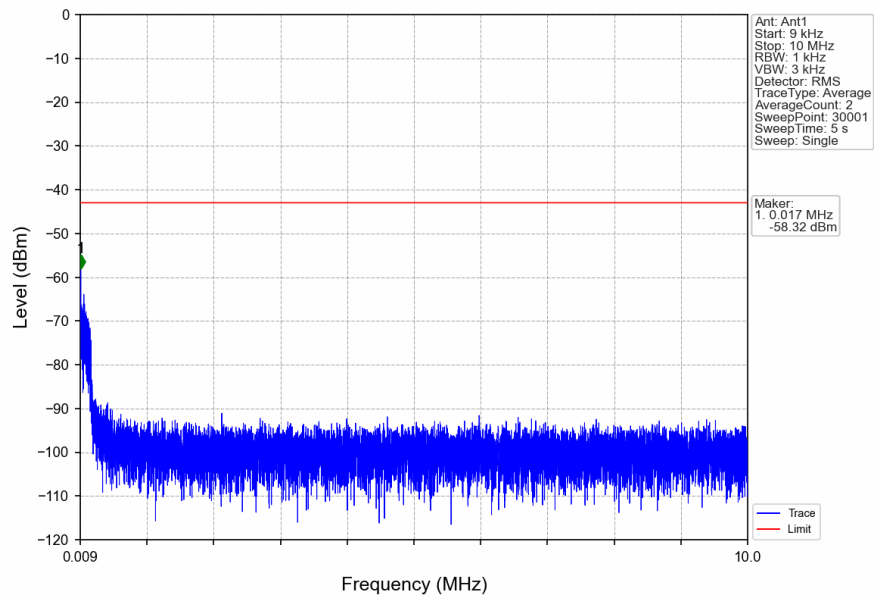
n5_15kHz_SISO_NTNV_20MHz_DFT-s-OFDM_QPSK_834MHz_Edge_1RB_Left
