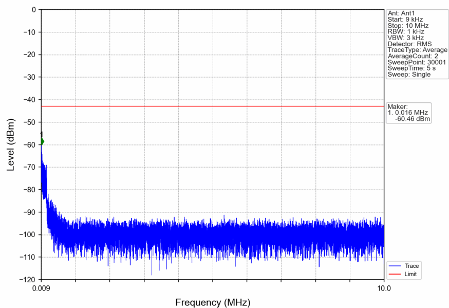
n5_15kHz_SISO_NTNV_20MHz_DFT-s-OFDM_QPSK_836.5MHz_Edge_1RB_Left
