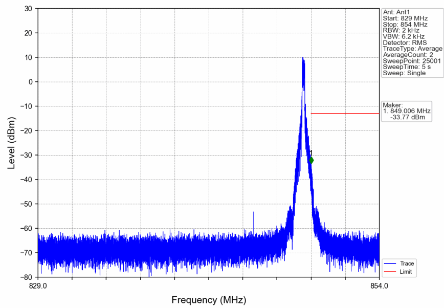
n5_15kHz_SISO_NTNV_20MHz_DFT-s-OFDM_PI/2_BPSK_839MHz_Edge_1RB_Right
