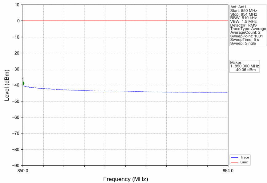
n5_15kHz_SISO_NTNV_15MHz_CP-OFDM_QPSK_841.5MHz_Inner_1RB_Right
