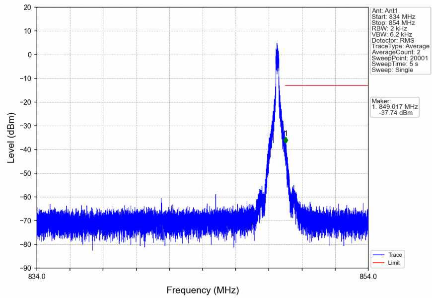
n5_15kHz_SISO_NTNV_15MHz_CP-OFDM_QPSK_841.5MHz_Edge_1RB_Right
