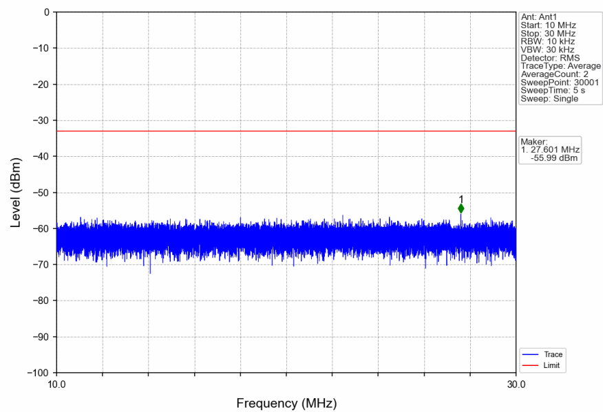
n5_15kHz_SISO_NTNV_20MHz_DFT-s-OFDM_QPSK_839MHz_Inner_1RB_Right
