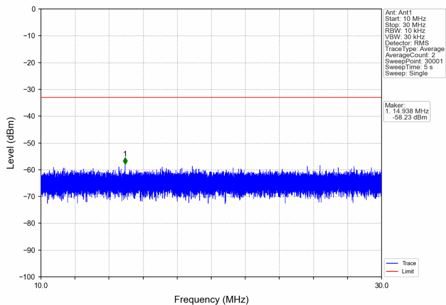
n5_15kHz_SISO_NTNV_20MHz_DFT-s-OFDM_QPSK_836.5MHz_Edge_1RB_Left
