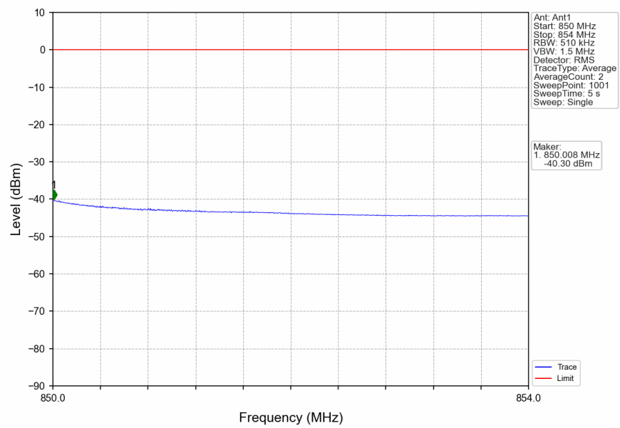
n5_15kHz_SISO_NTNV_20MHz_DFT-s-OFDM_QPSK_839MHz_Inner_1RB_Right
