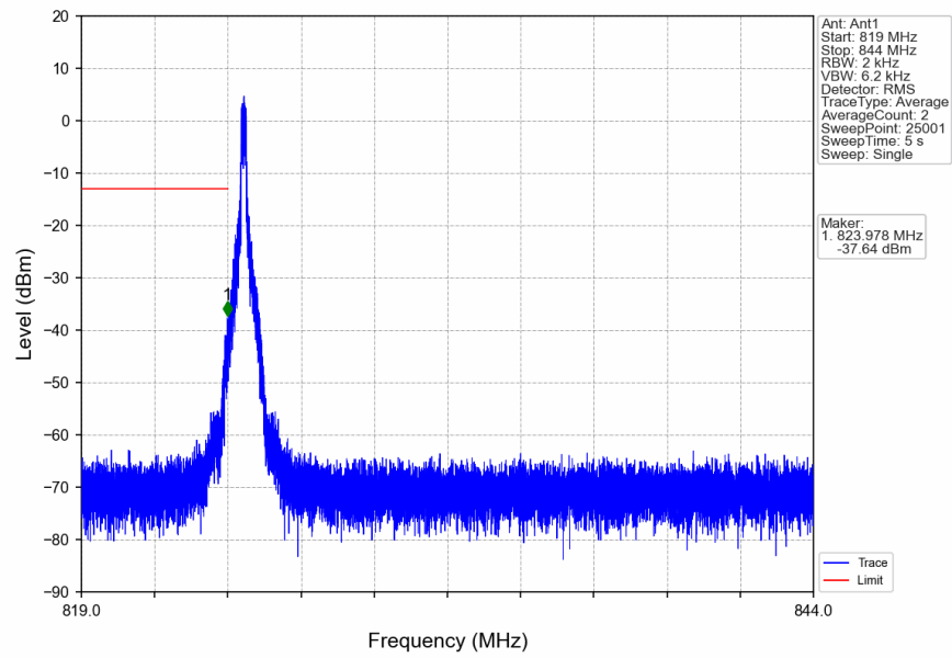
n5_15kHz_SISO_NTNV_20MHz_CP-OFDM_QPSK_834MHz_Edge_1RB_Left
