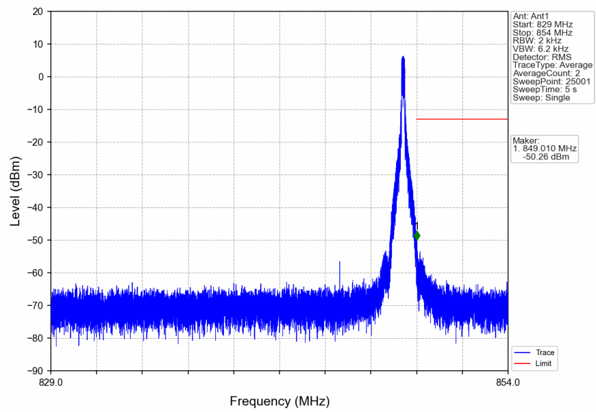
n5_15kHz_SISO_NTNV_20MHz_DFT-s-OFDM_QPSK_839MHz_Inner_1RB_Right
