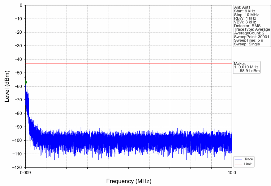
n5_15kHz_SISO_NTNV_20MHz_DFT-s-OFDM_QPSK_839MHz_Inner_1RB_Right
