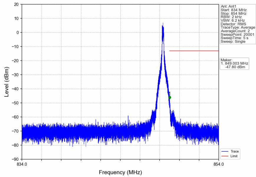
n5_15kHz_SISO_NTNV_15MHz_CP-OFDM_QPSK_841.5MHz_Inner_1RB_Right
