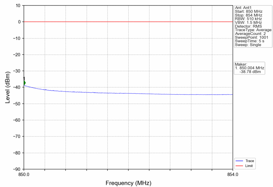
n5_15kHz_SISO_NTNV_20MHz_DFT-s-OFDM_QPSK_839MHz_Edge_1RB_Right
