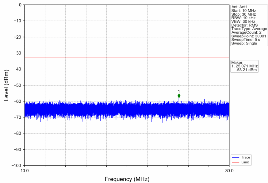
n5_15kHz_SISO_NTNV_20MHz_DFT-s-OFDM_QPSK_834MHz_Edge_1RB_Left
