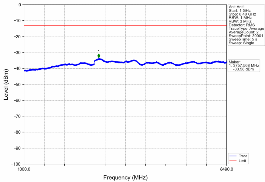
n5_15kHz_SISO_NTNV_20MHz_CP-OFDM_QPSK_834MHz_Outer_Full
