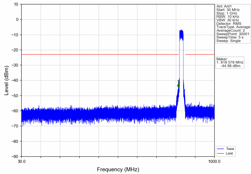
n5_15kHz_SISO_NTNV_20MHz_CP-OFDM_QPSK_834MHz_Outer_Full
