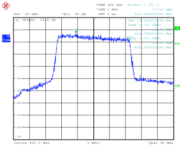
QPSK Low channel
