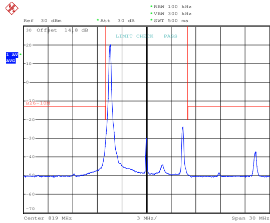
QPSK Middle channel-1 RB offset 0
