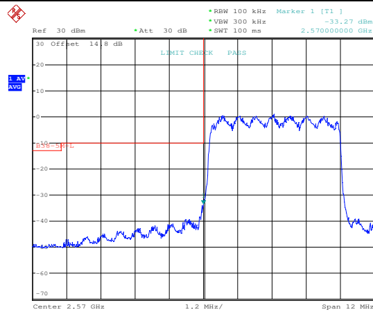
QPSK Low channel-25 RB offset 0
