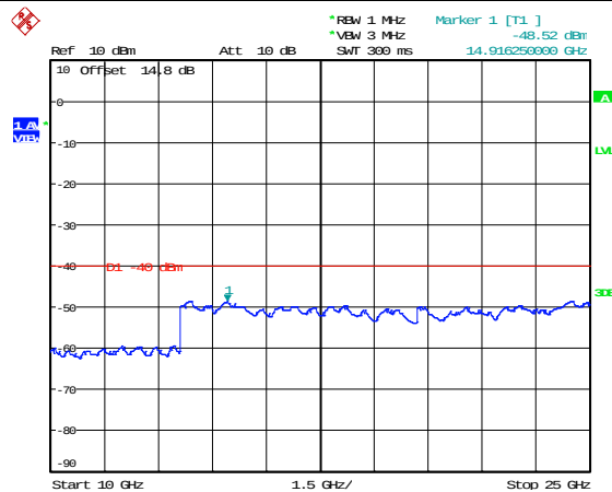
QPSK High channel-10GHz~25GHz
