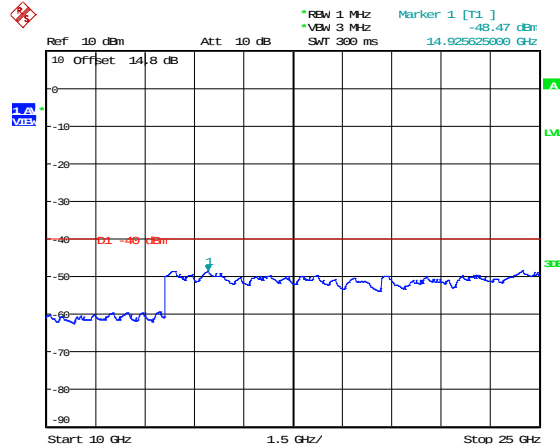
QPSK Low channel-10GHz~25GHz
