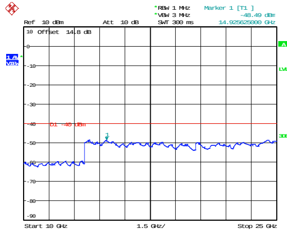
QPSK Middle channel-10GHz~25GHz
