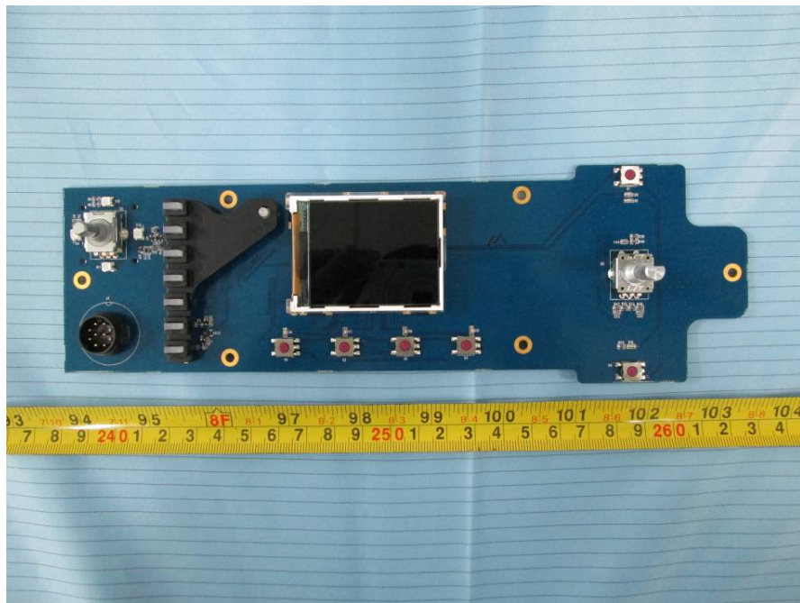
EUT – LCD & Key Board Top View
