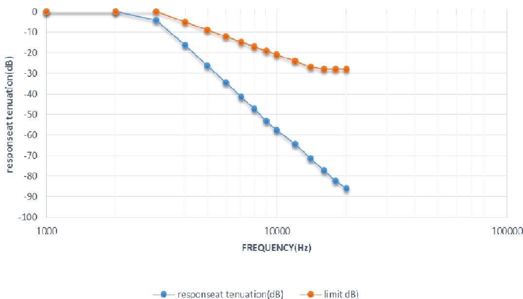
151.125MHz, 25KHz , Audio Low Pass Filtr Response
