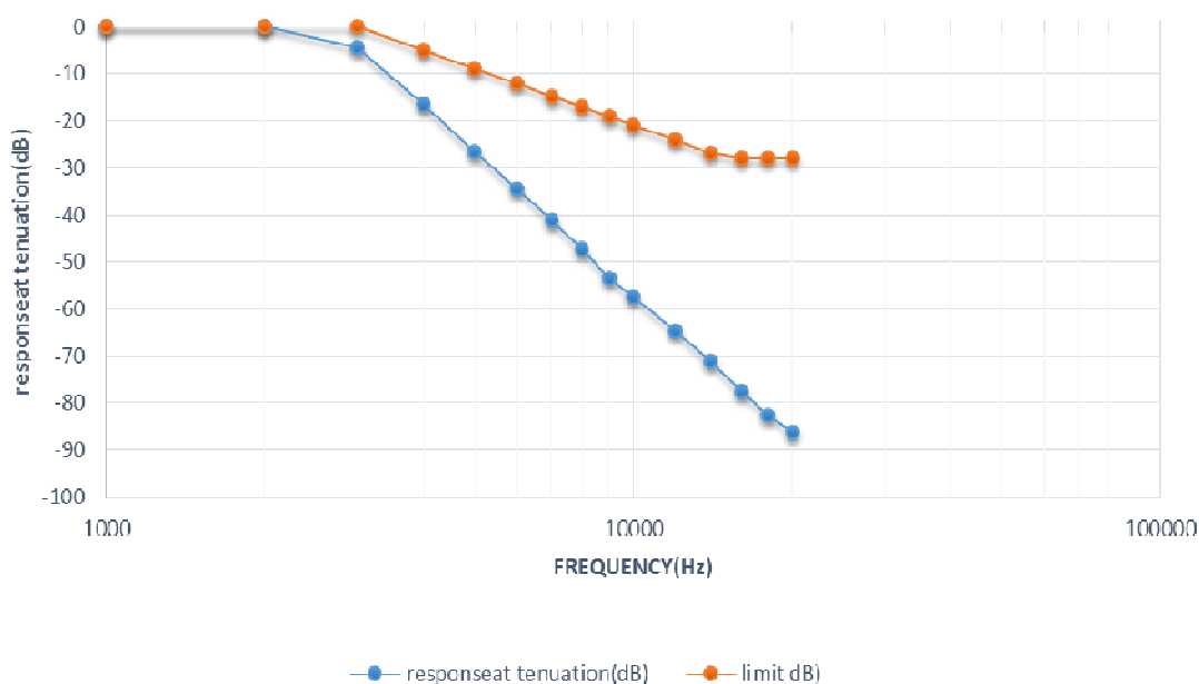
158.125MHz, 25KHz , Audio Low Pass Filtr Response
