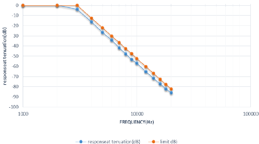
158.125MHz, 12.5KHz , Audio Low Pass Filtr Response
