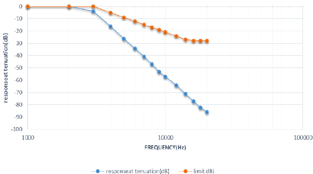
173.875MHz, 25KHz , Audio Low Pass Filtr Response
