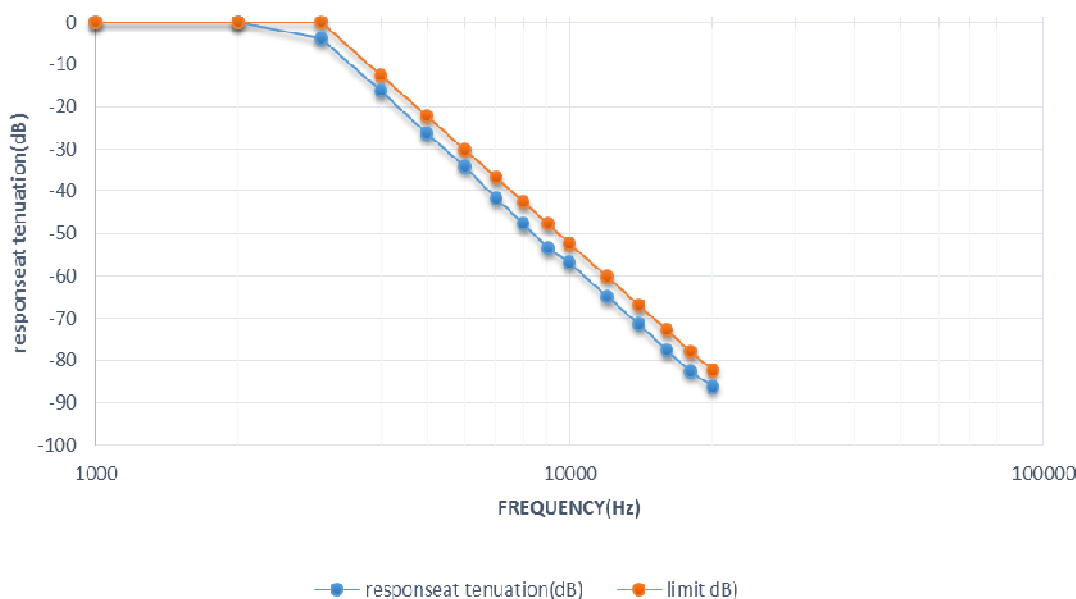
151.125MHz, 12.5KHz , Audio Low Pass Filtr Response
