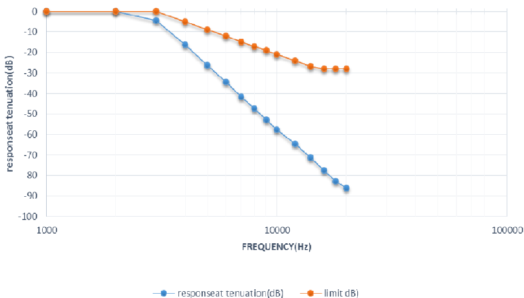
136.125MHz, 25KHz , Audio Low Pass Filtr Response
