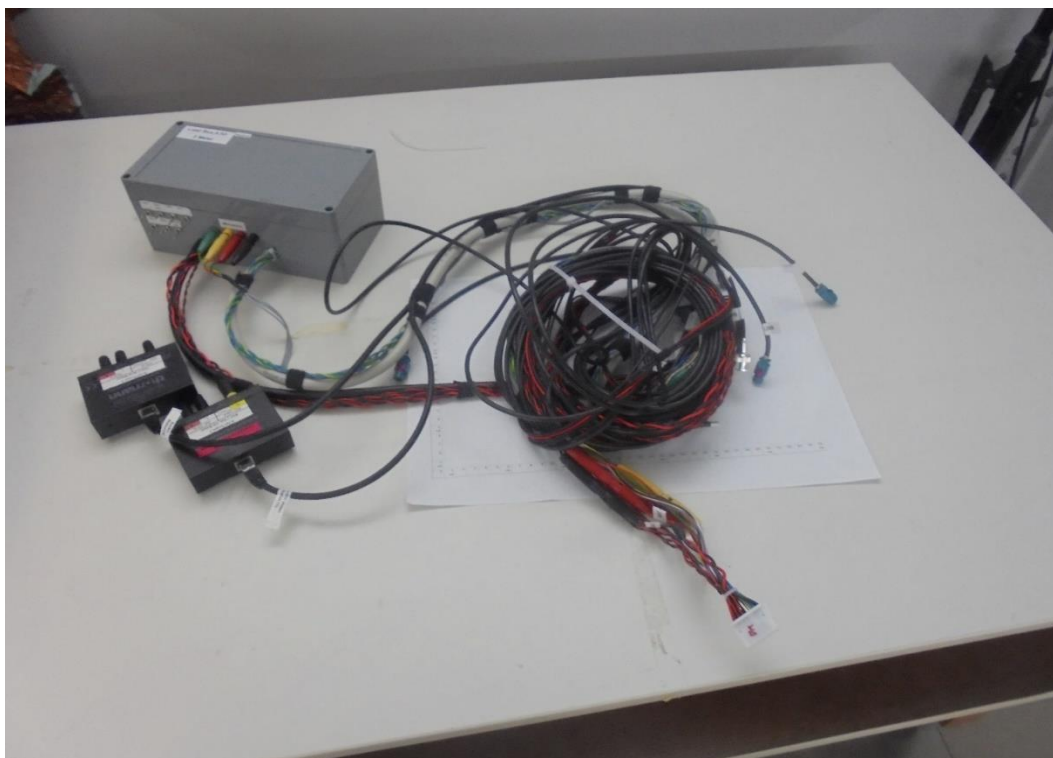
Photograph 12: Load box with 2 Meter Harness
