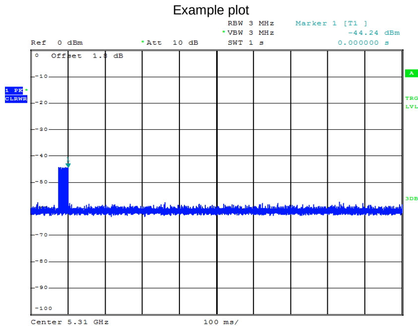
Plot 3
