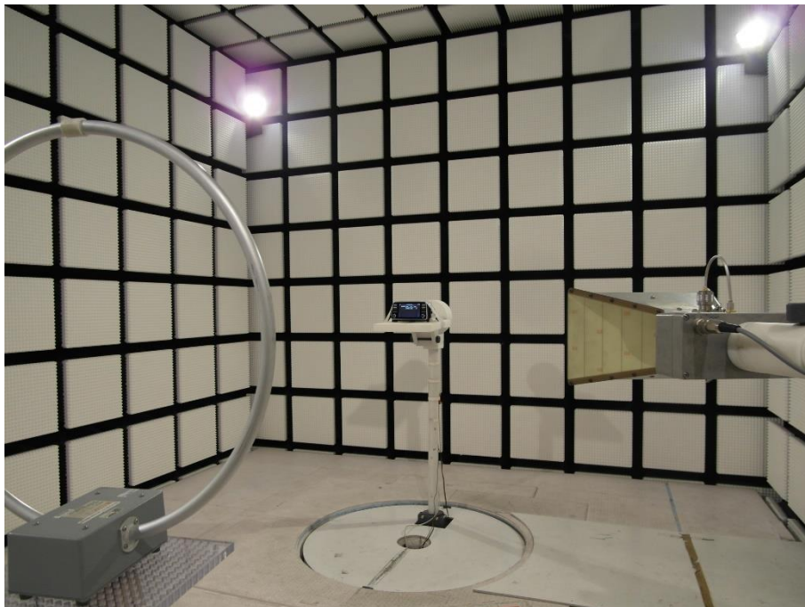
Photo 6: RSE set-up (>1GHz)
