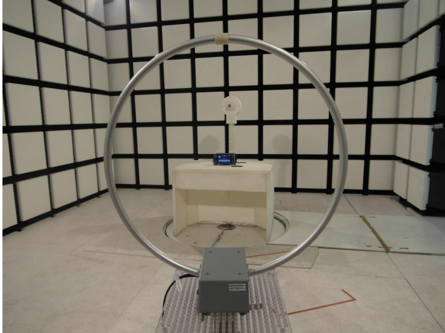
Photo 9: RSE set-up (<30MHz)
