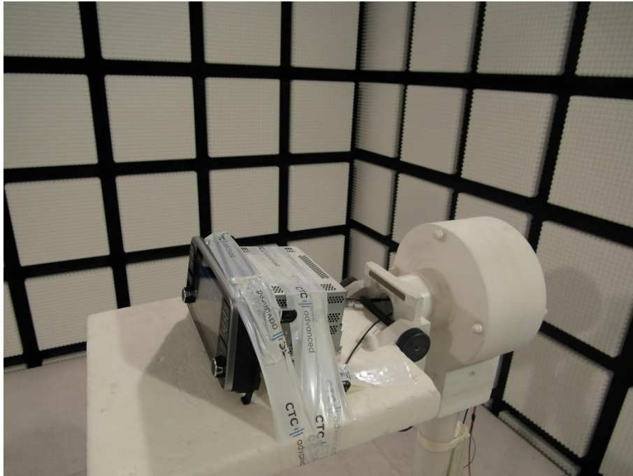
Photo 7: RSE set-up (>1GHz)
