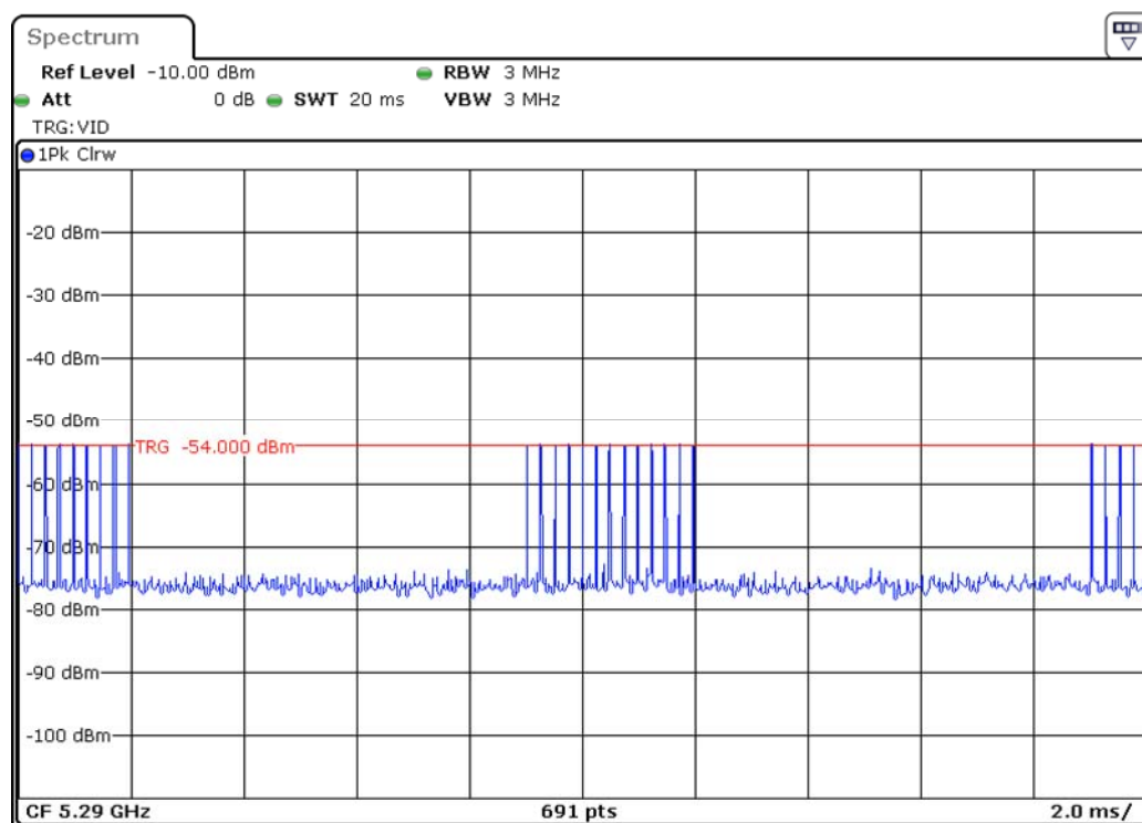
Radar Type 4 Calibration Plot (5290MHz)
