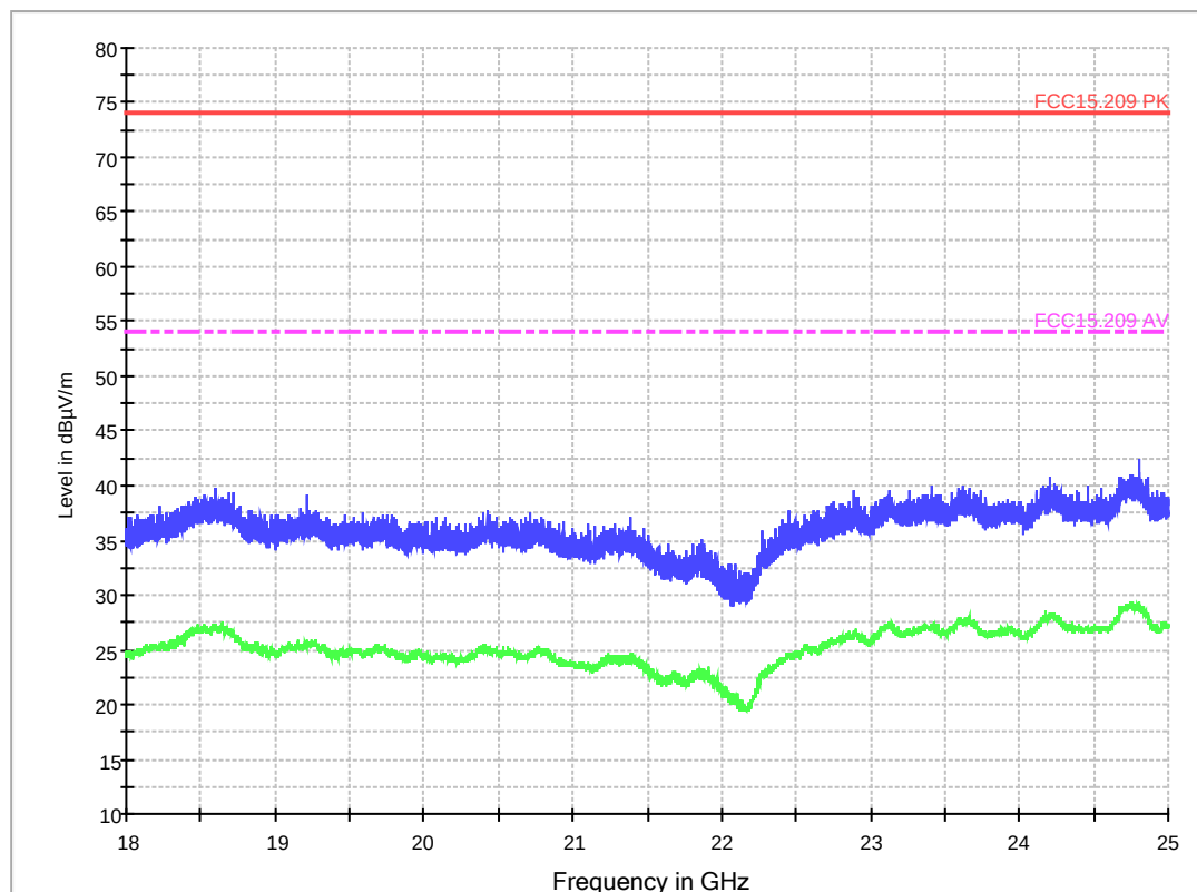
EMI Scan_18_25GHz_Pre
