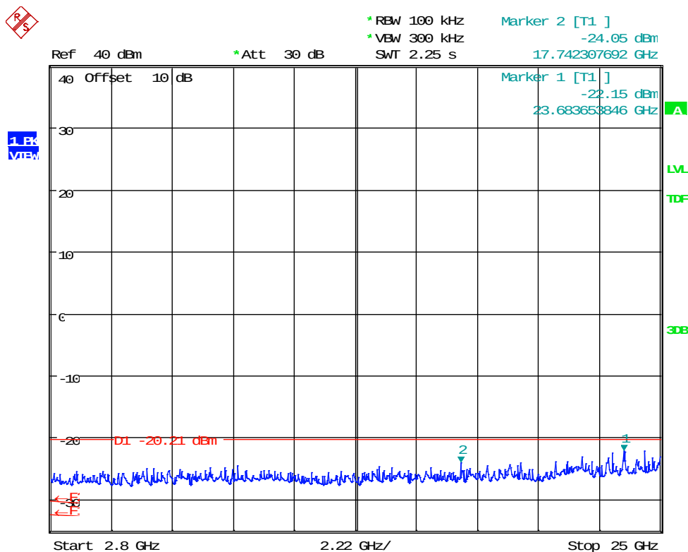
Plot 33: 20dBc | 2.8-25GHz | 3-DH3 | 8 DQPSK | Ch 78 (2480 MHz)
