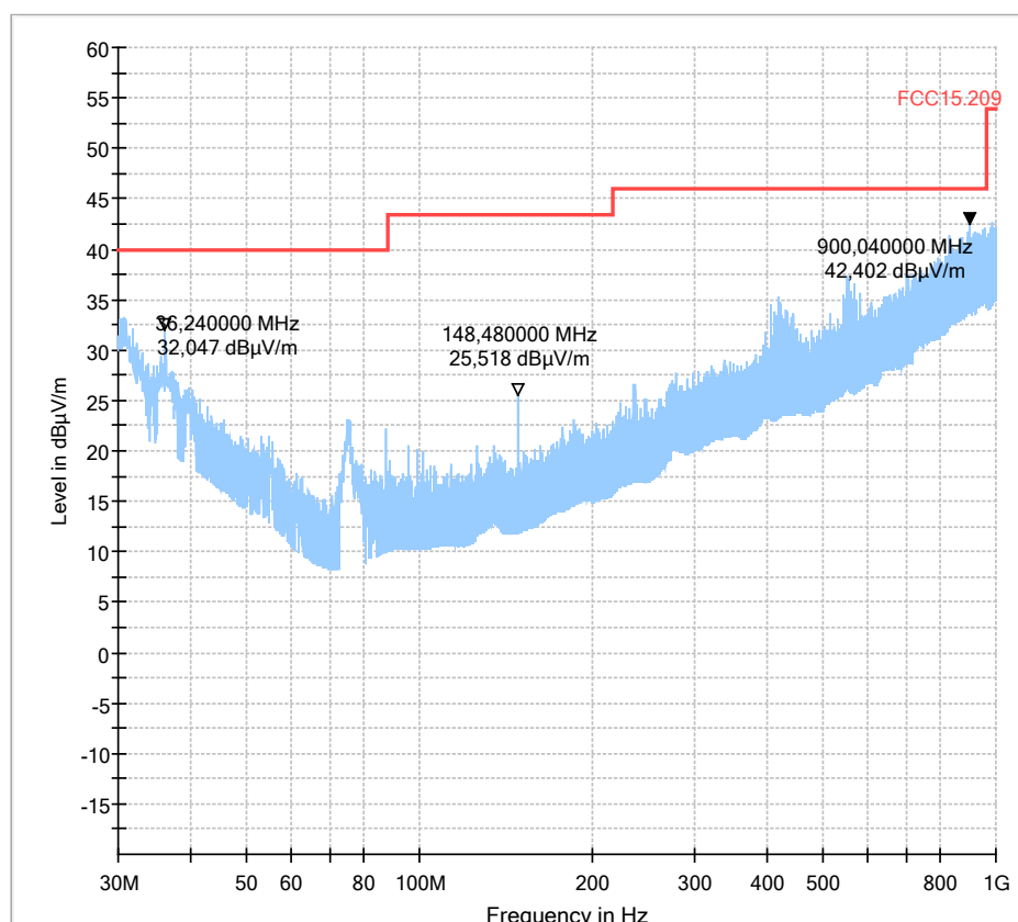
Full Spectrum
