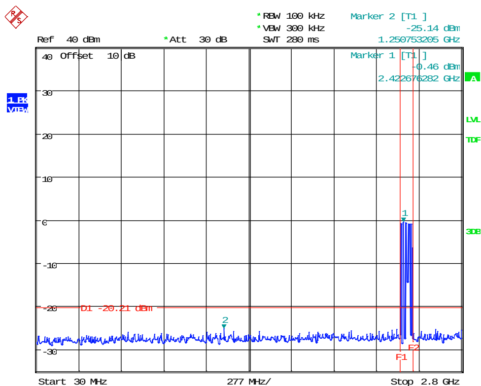
Plot 32: 20dBc | 30MHz-2.8GHz | 3-DH3 | 8 DQPSK | Ch 78 (2480 MHz)
