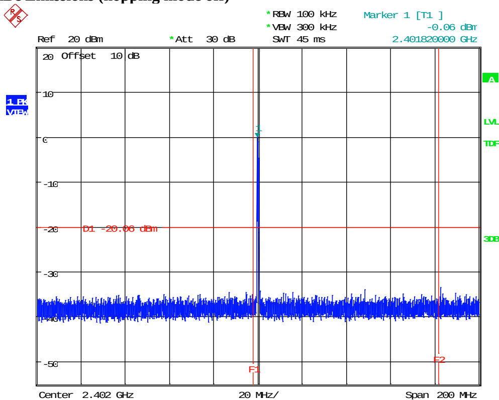
Plot 10: 20dBc Ref | DH1 | GFSK | Ch 0 (2402 MHz)
