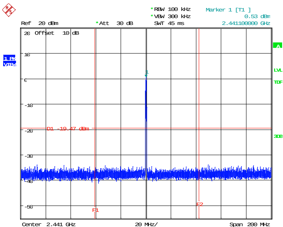
Plot 14: 20dBc Ref | 2-DH5 | pi/4 DQPSK | Ch 39 (2441 MHz)
