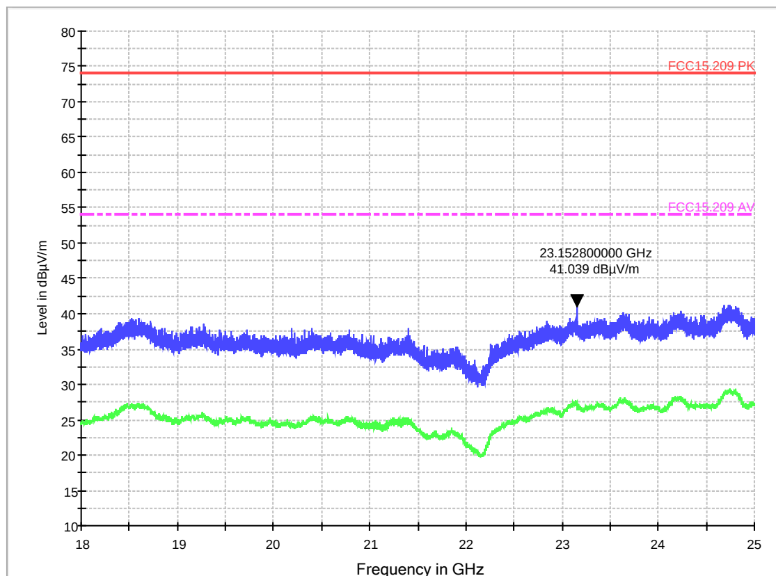
EMI Scan_18_25GHz_Pre
