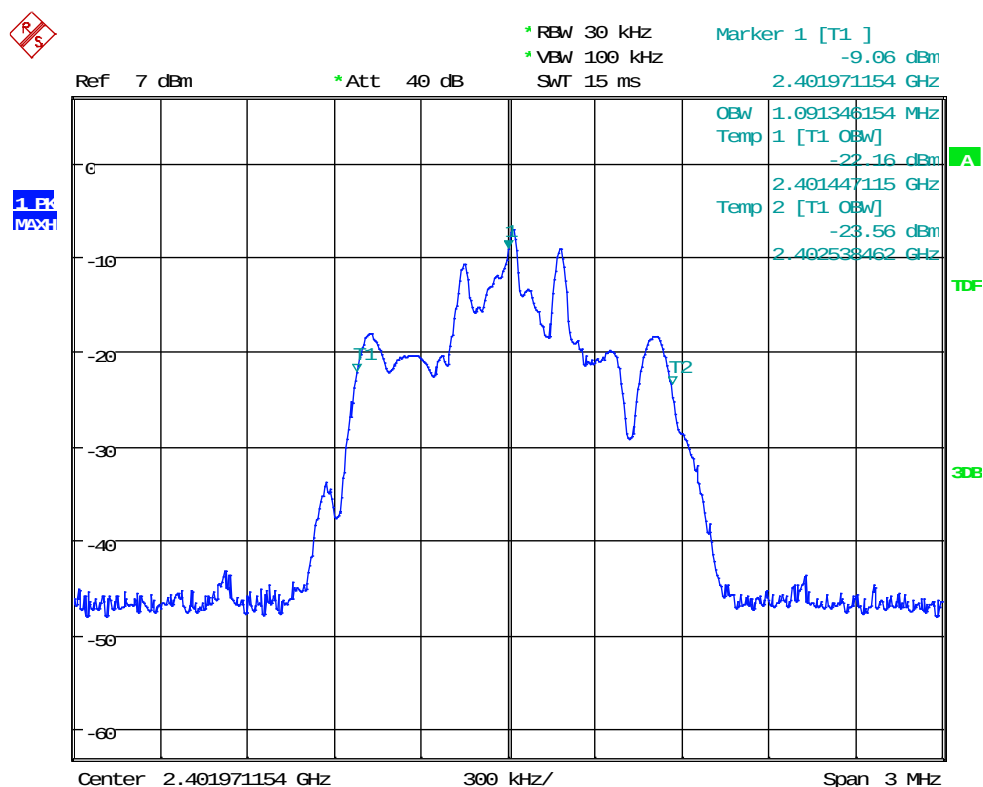
Plot 7: 99%BW_BT_3-DH3_ch00
