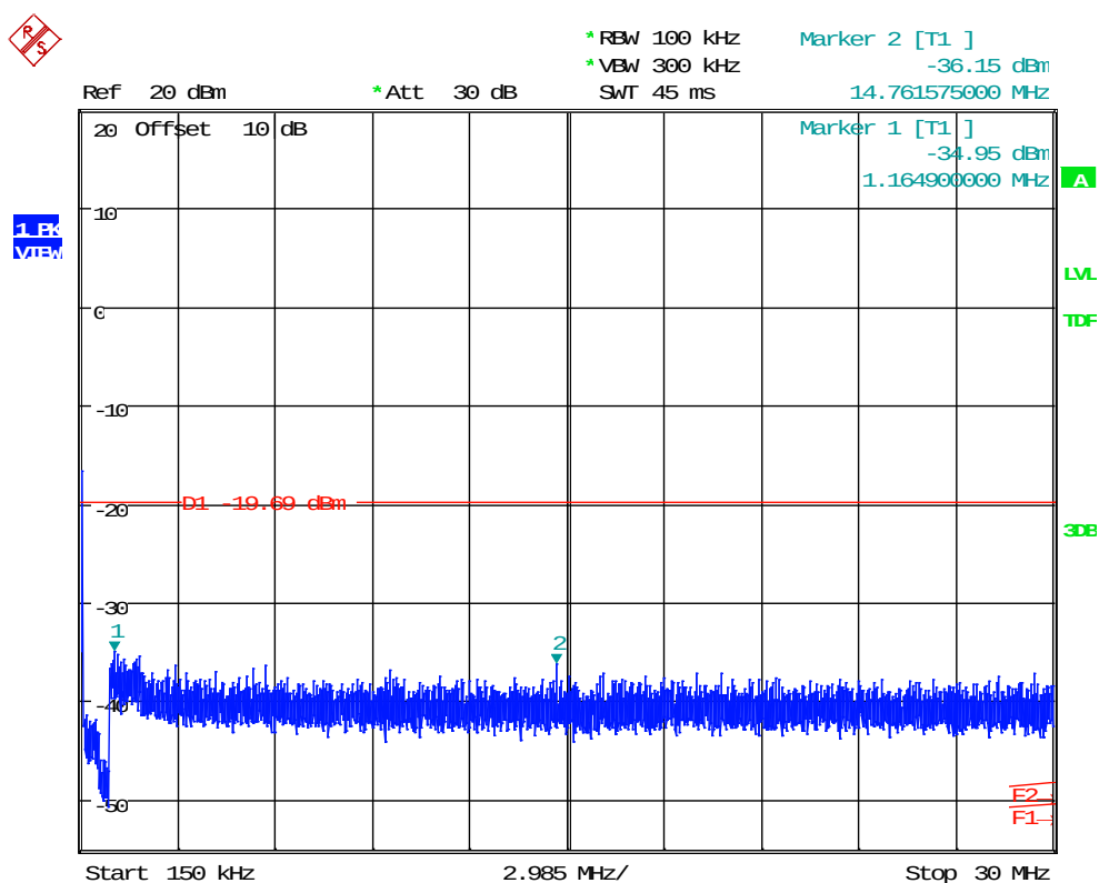
Plot 19: 20dBc | 0.15-30MHz | 3-DH3 | 8 DQPSK | Ch 78 (2480 MHz)
