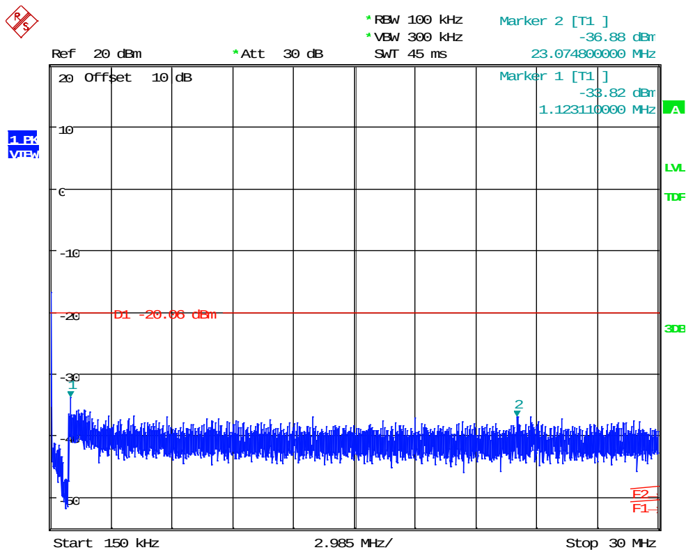
Plot 11: 20dBc | 0.15-30MHz || DH1 | GFSK | Ch 0 (2402 MHz)
