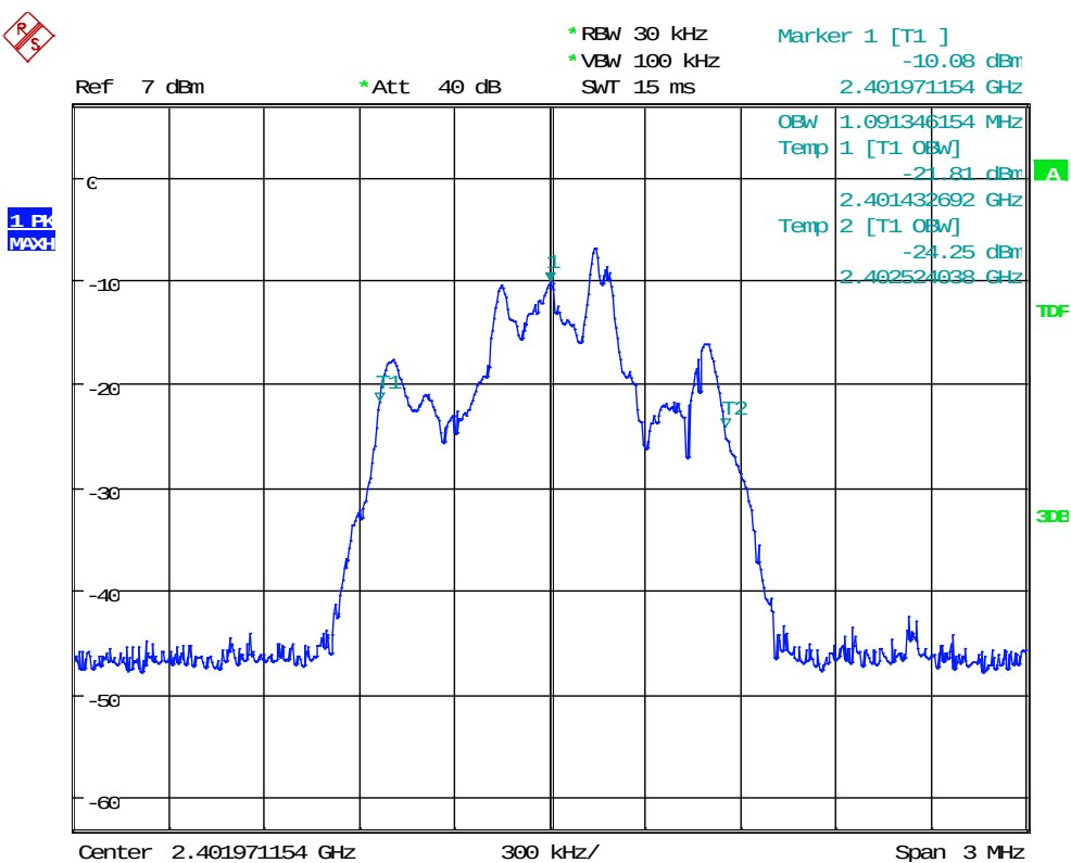
Plot 4: 99%BW_BT_2-DH5_ch00
