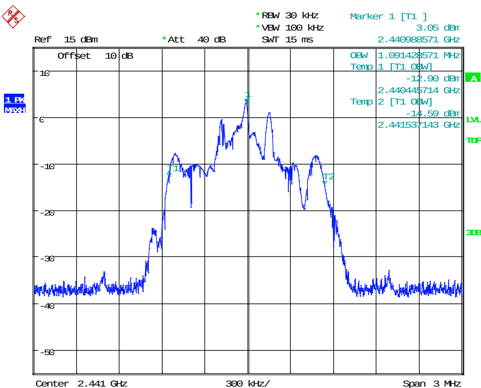
Plot 8: 99%BW_BT_3-DH3_ch39
