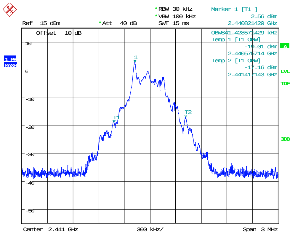
Plot 2: 99%BW_BT_DH1_ch39
