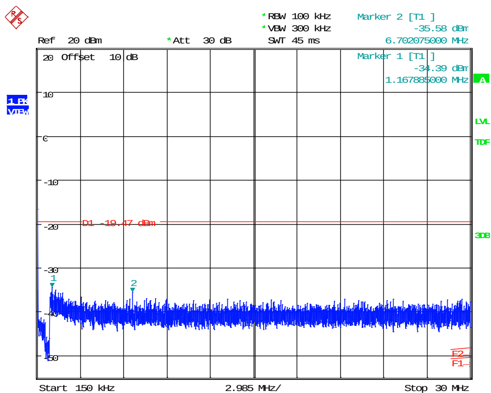
Plot 15: 20dBc | 0.15-30MHz | 2-DH5 | pi/4 DQPSK | Ch 39 (2441 MHz)
