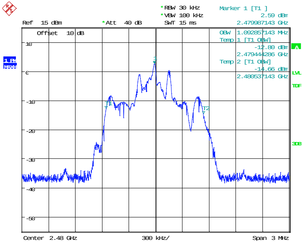
Plot 9: 99%BW_BT_3-DH3_ch78
