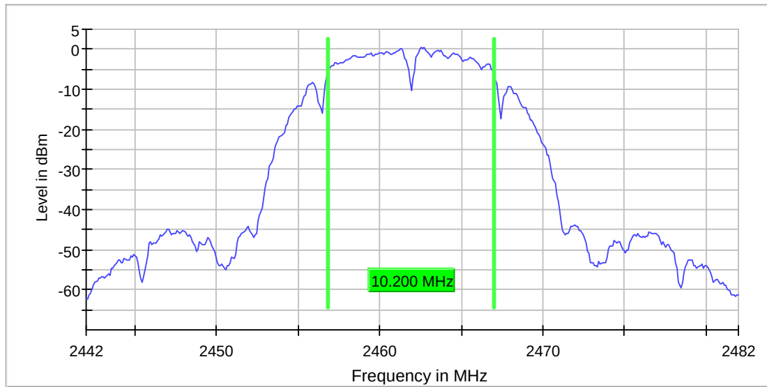
6dB_BW_CH11_bmode_2MBIT
