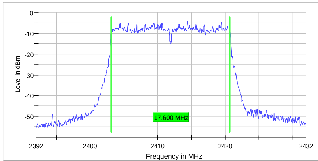
99% Occupied Bandwidth CH1_n mode_MCS3
