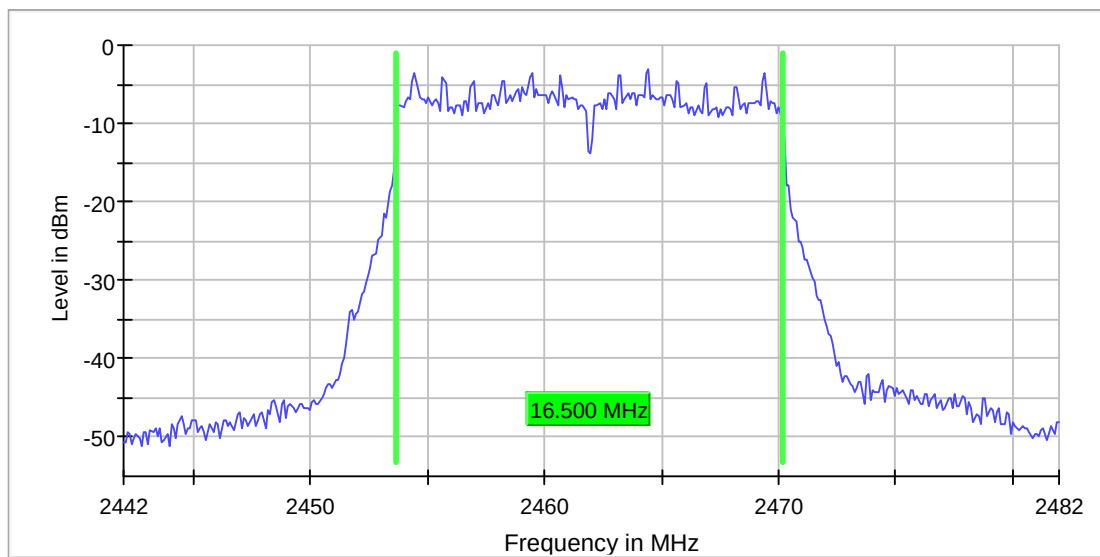
6dB_BW_CH11_g-mode_6MBIT
