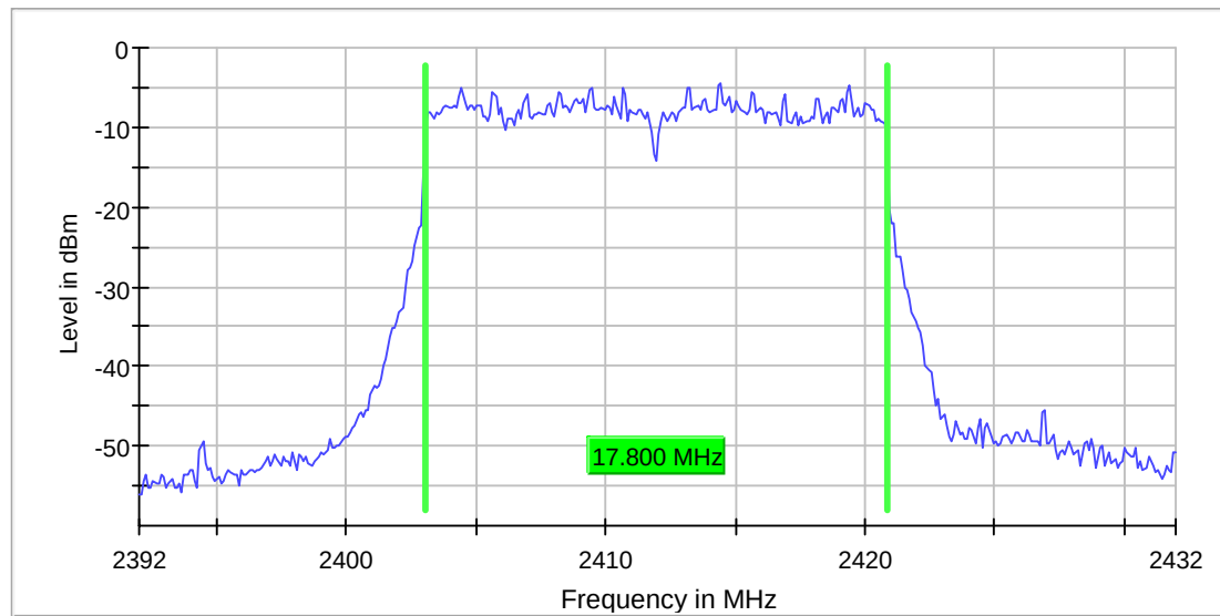
6dB_BW_CH01_n-mode_MCS3
