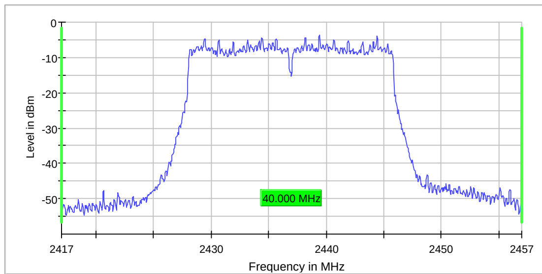
99% Occupied Bandwidth CH6_n mode_MCS3
