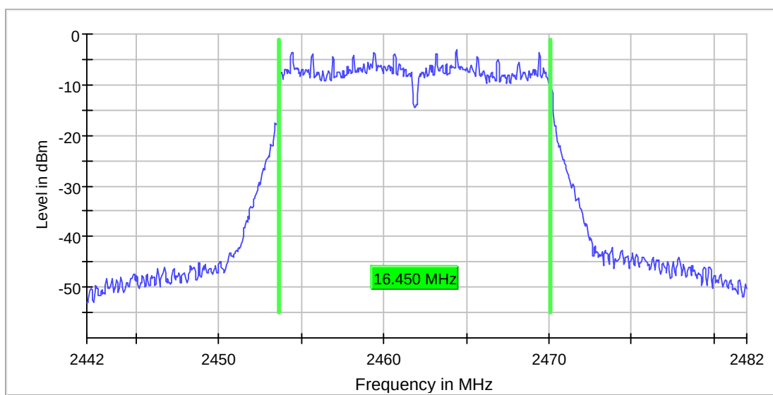
99% Occupied Bandwidth CH11_g mode_6Mbit
