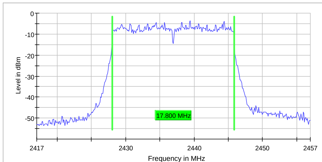
6dB_BW_CH06_n-mode_MCS3
