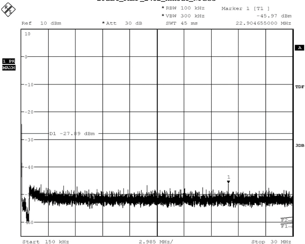
20dBc_0.15MHz-30MHz_2462_nmode_MCS3
