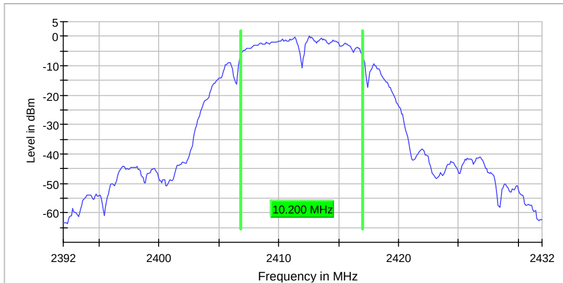
6dB_BW_CH01_bmode_2MBIT
