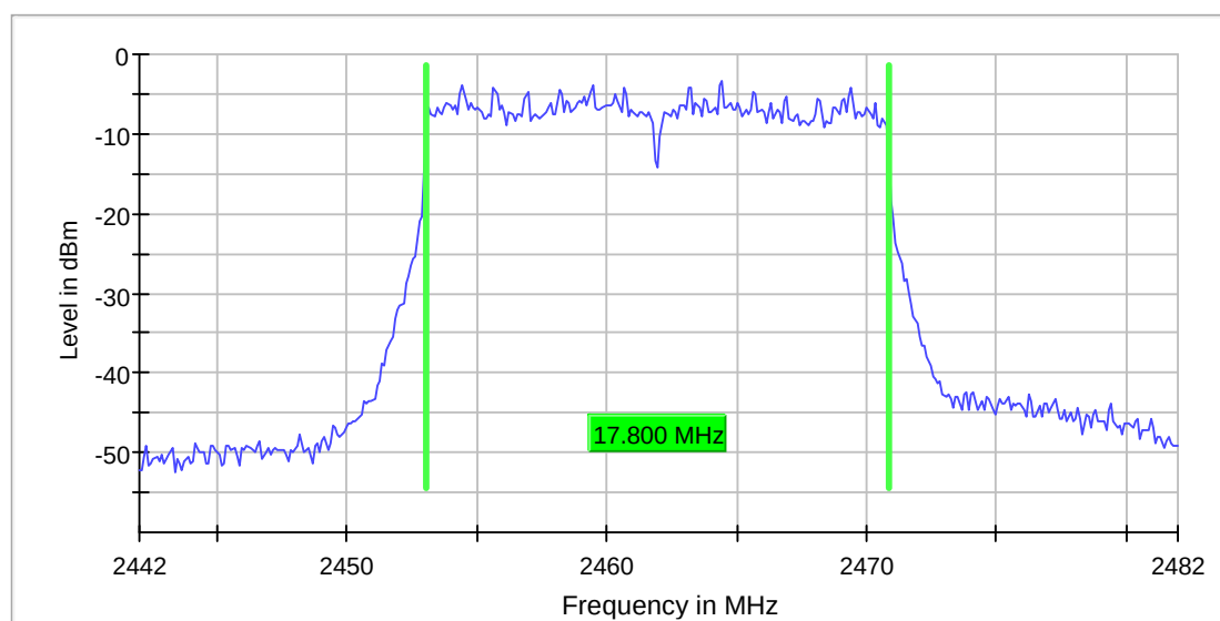
6dB_BW_CH11_n-mode_MCS3
