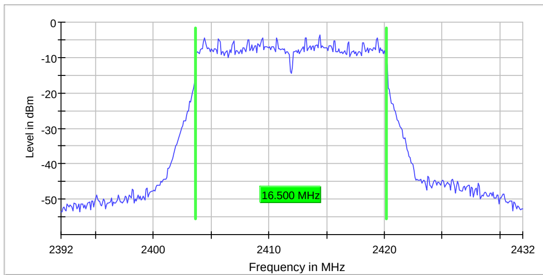
6dB_BW_CH01_g-mode_6MBIT
