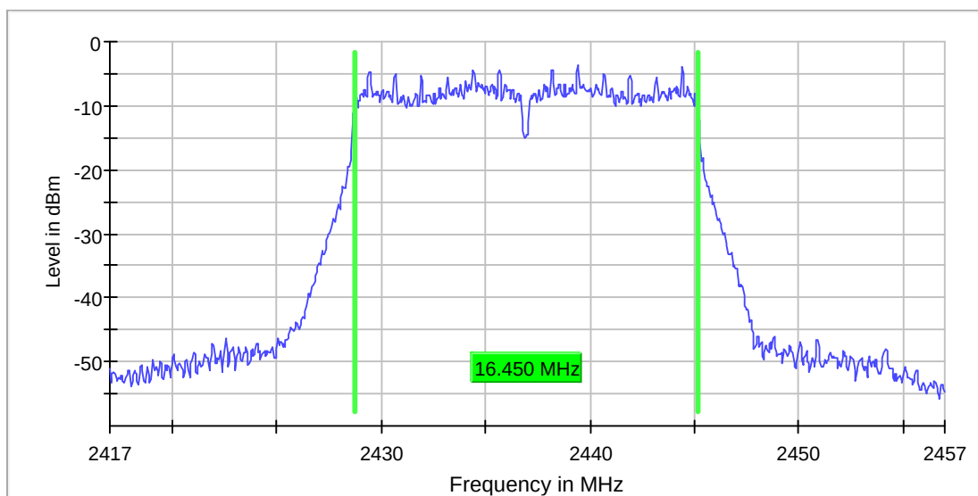
99% Occupied Bandwidth CH6_g mode_6Mbit
