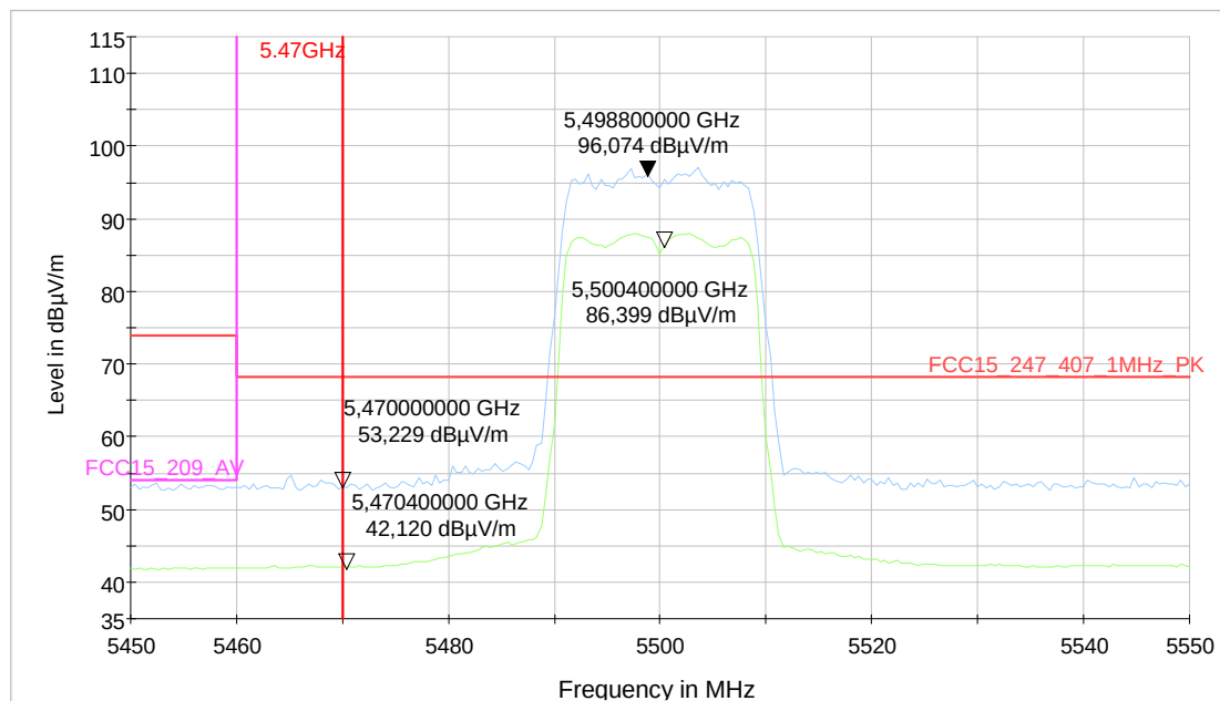
9.11a_ac-mode_MCS4_ch100
