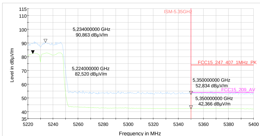
9.17b_ac-mode_MCS0_ch046
