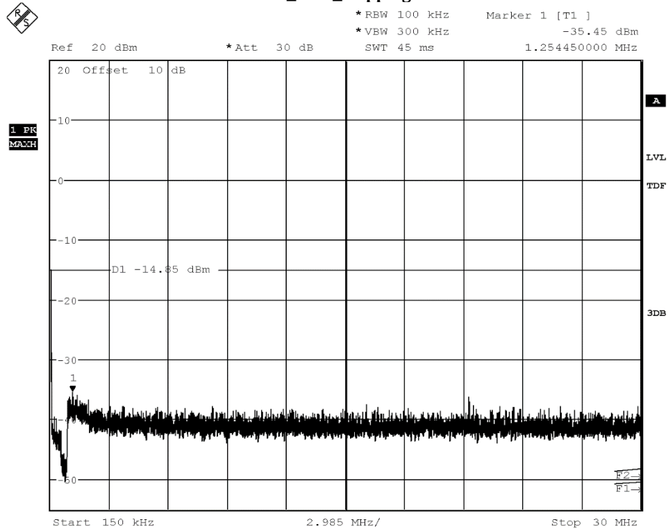
20dBc_0.15MHz-30MHz_Hopping ON
