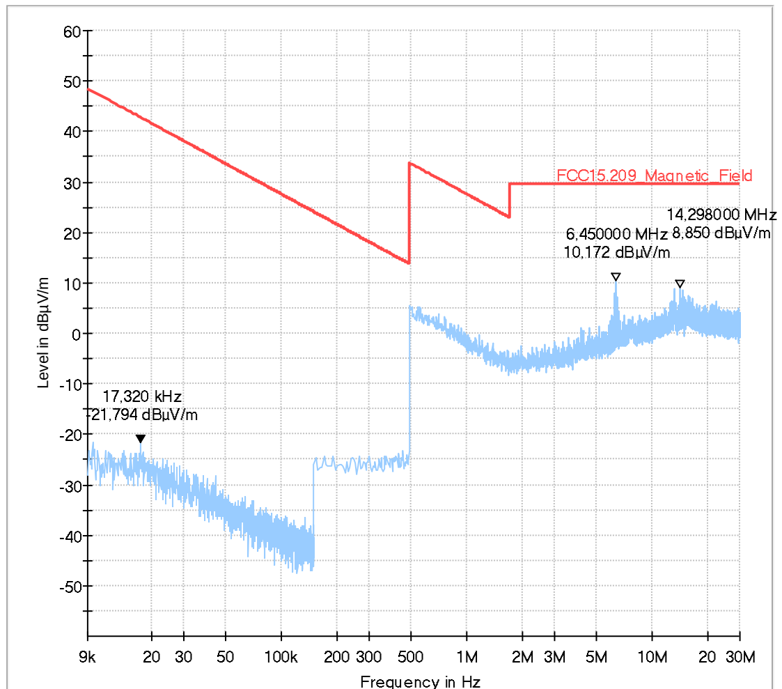
Full Spectrum
