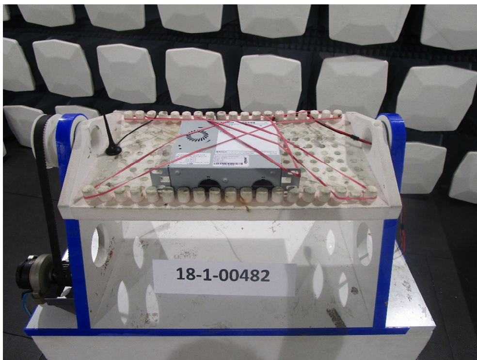
Photograph 9: Close View above 1GHz- EUT Laying
