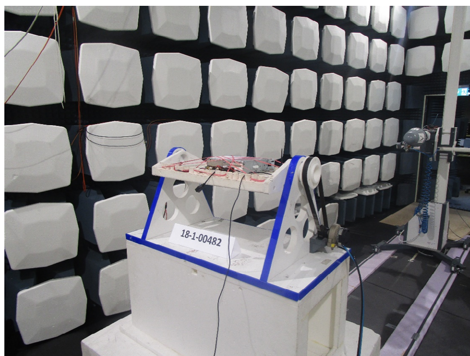
Photograph 10: Overall View 1 GHz-18 GHz - EUT Laying
