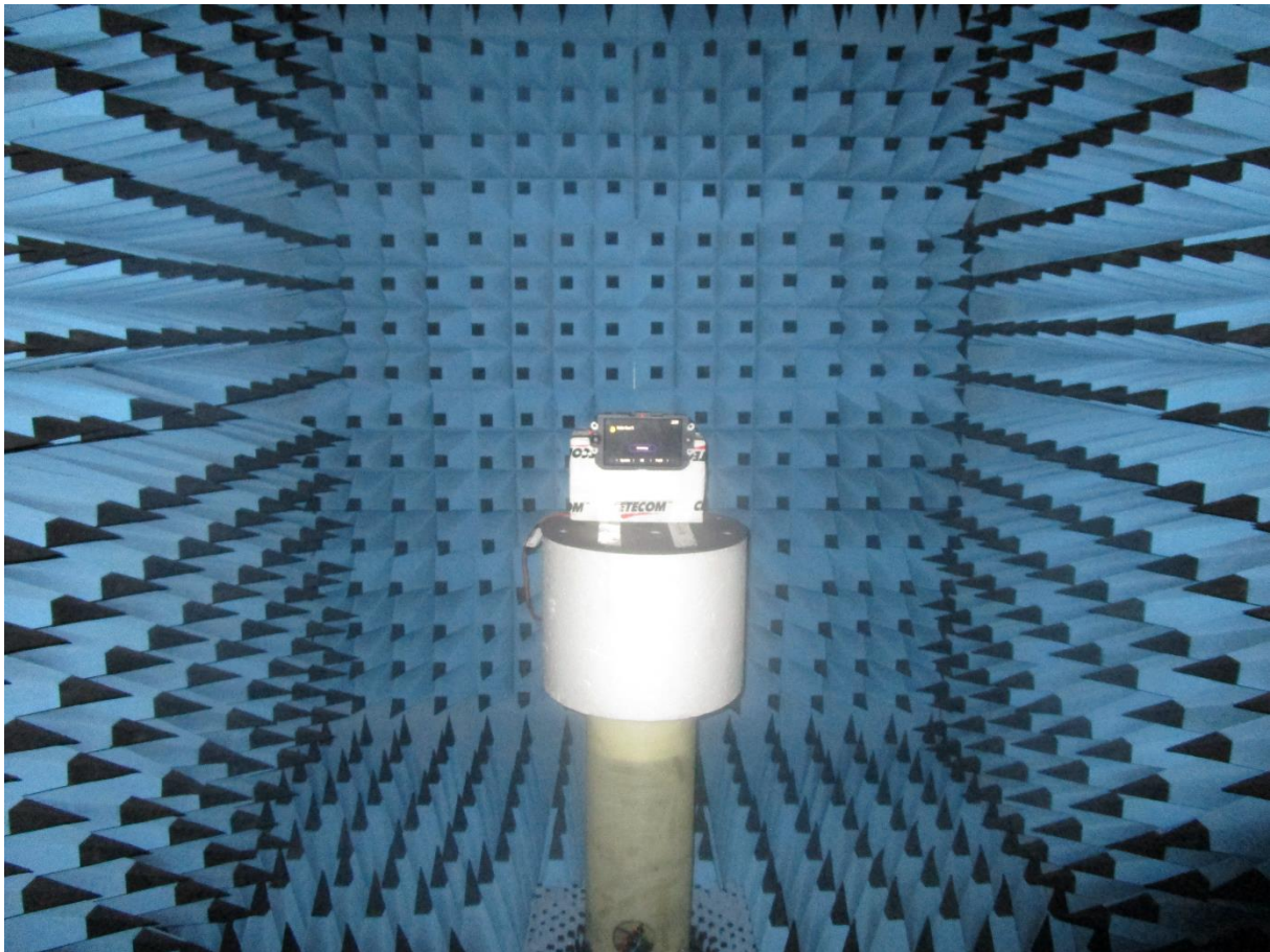
Photograph 1: Free Space setup (FS), long shot view, \Theta=0^\circ , \Phi=0^\circ
