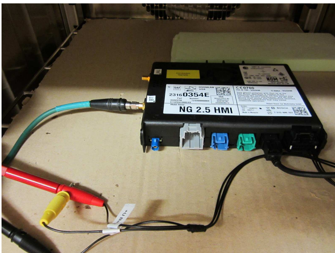
Photo 5: Test setup for conducted measurements
