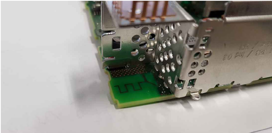
BT Antenna
