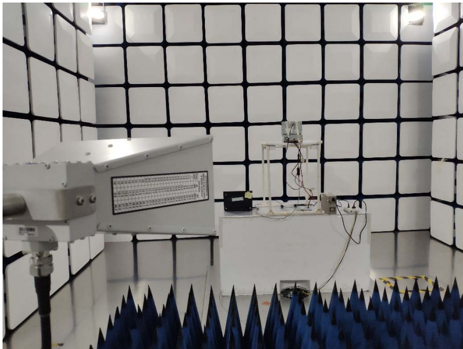
Above 1GHz-BT
