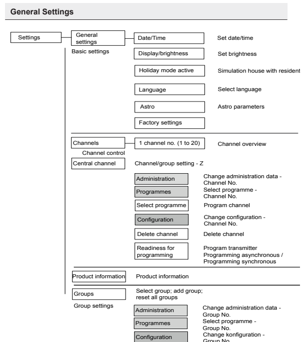
Fig. 6 Menu structure general settings
