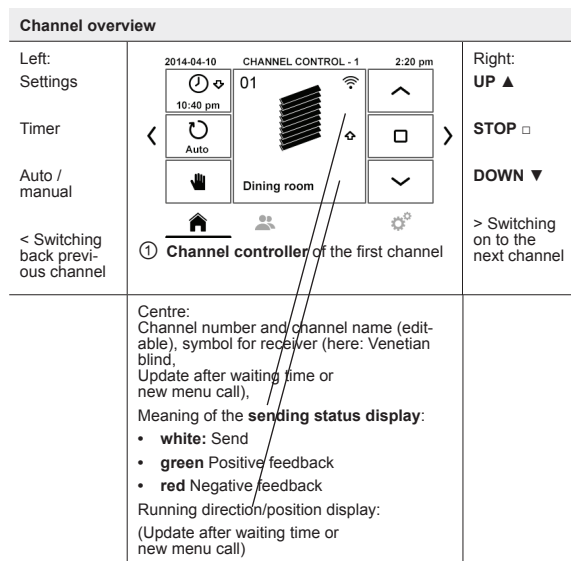
Fig. 3 Channel control channel 1
