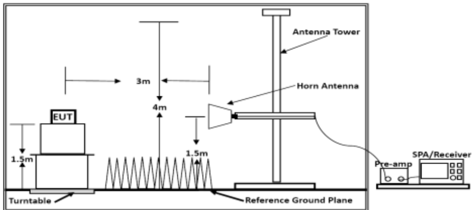
Above 1GHz
