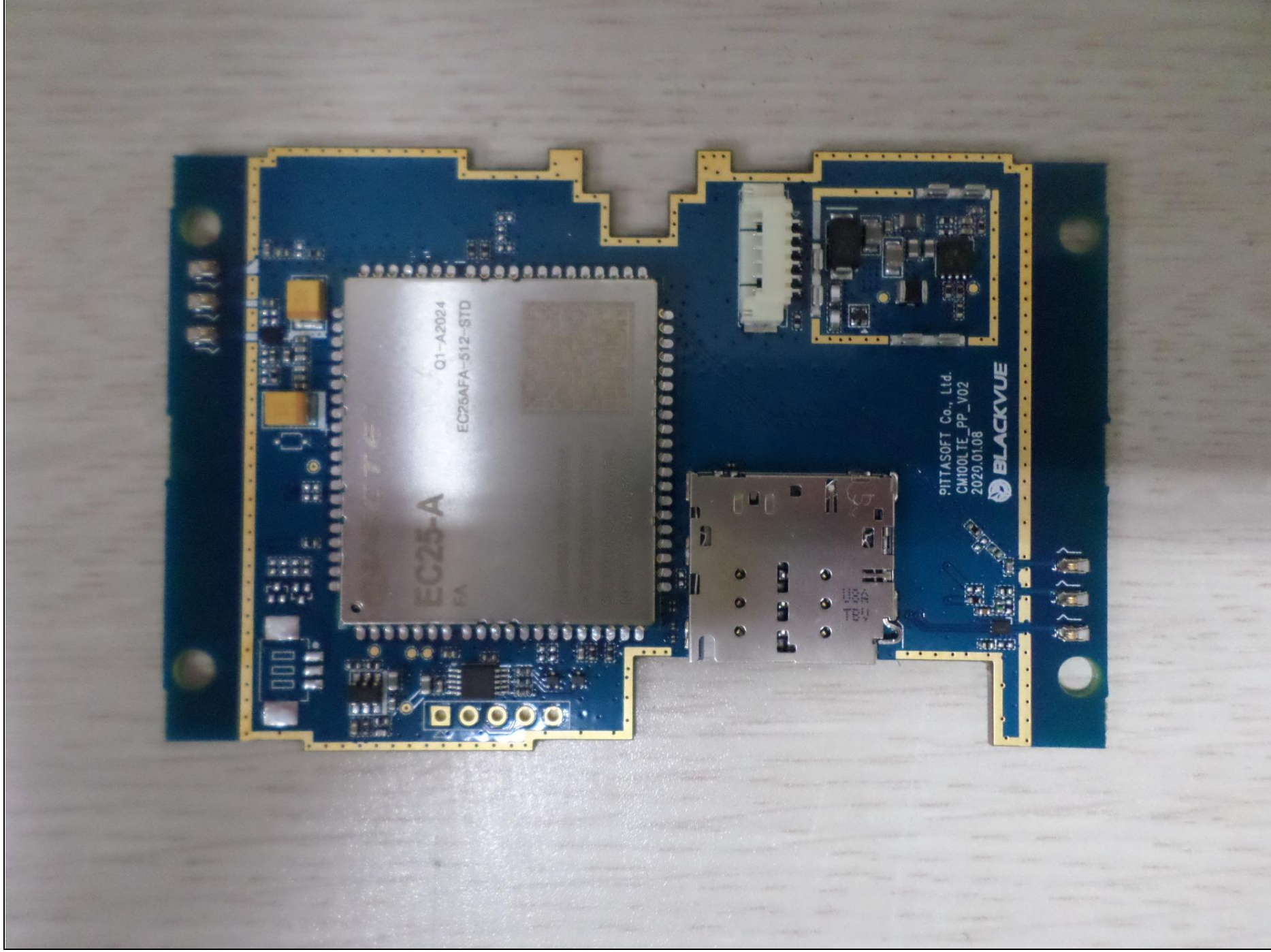
Front View of Main Board
