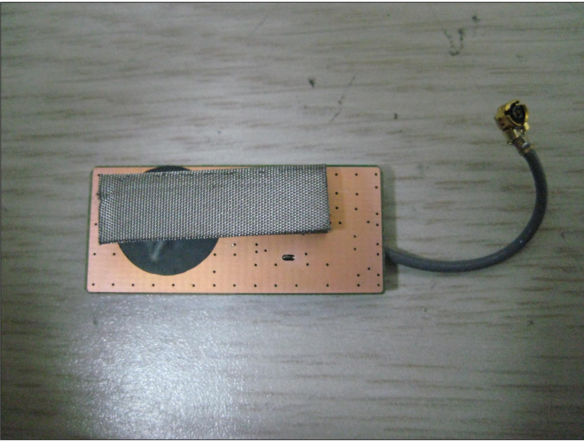
Rear View of Module
