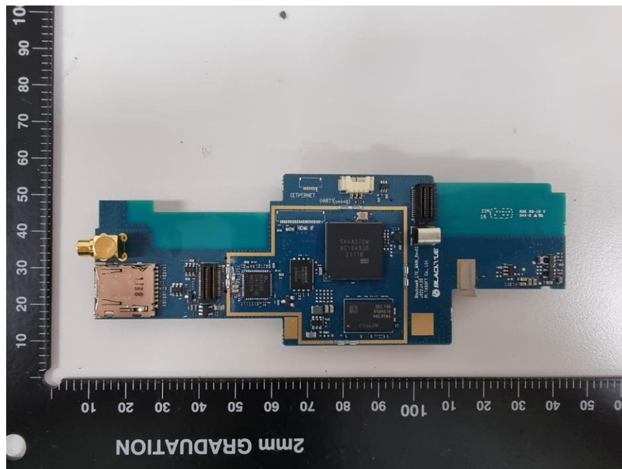
Sub board (Remove shield) - Front Top
