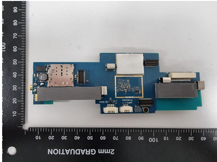
Sub board - Rear Bottom
