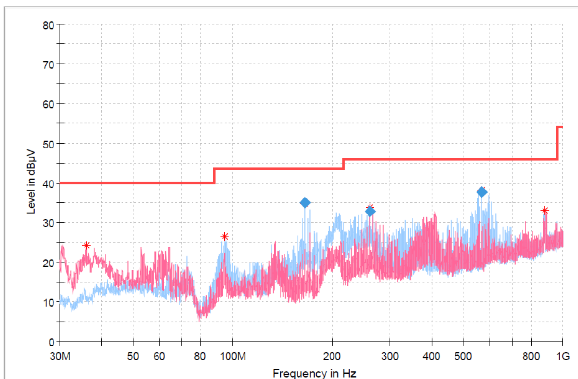
Worst case – RSE (Below 1 GHz)_TM 1
