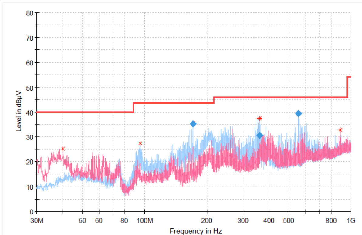
Worst case – RSE (Below 1 GHz)_TM 1_SISO (NII 1)
