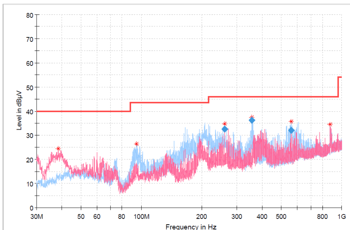
Worst case – RSE (Below 1 GHz)_TM 2
