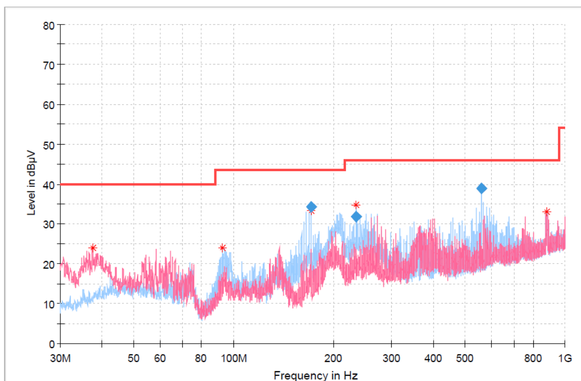
Worst case – RSE (Below 1 GHz)_TM 1
