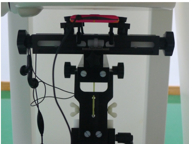
Back of the DUT with Phantom 1 cm Gap for Headset
