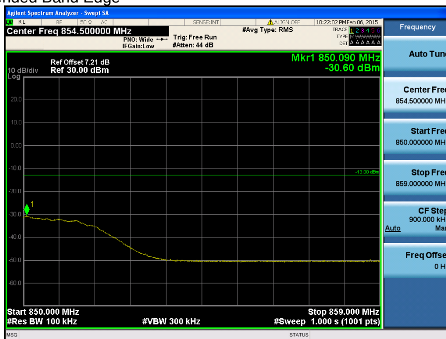
LTE Band 26 / 10MHz / QPSK - RB Size/Offset (50/0)
