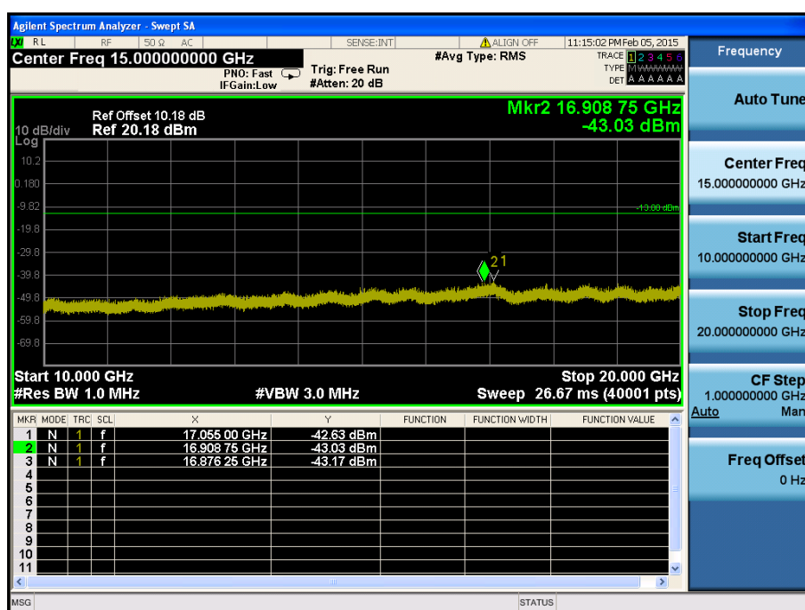
LTE Band 25 / 20MHz / 16QAM - RB Size/Offset (1/0) – High Channel
