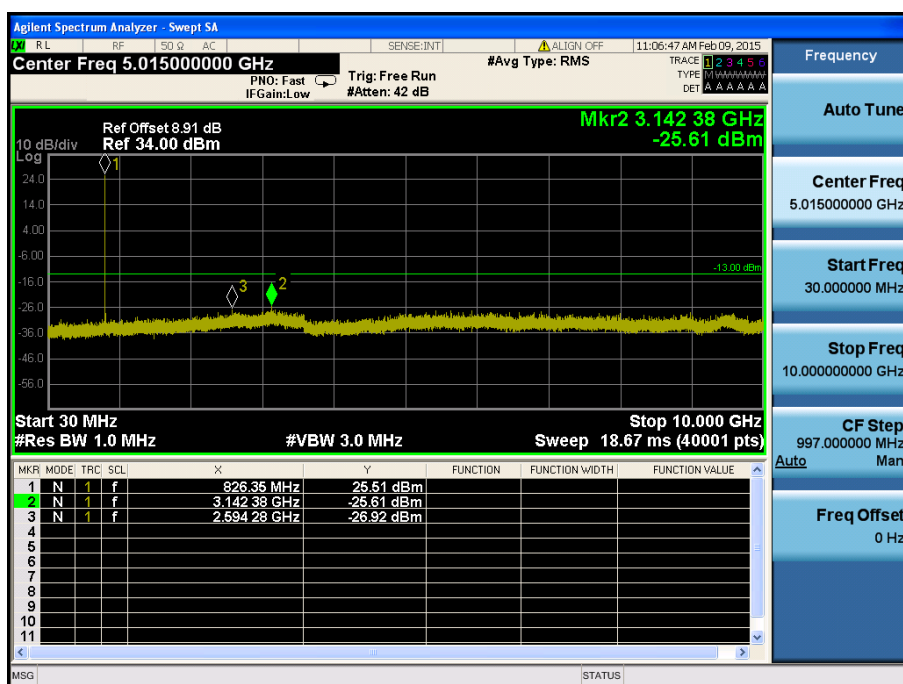
LTE Band 26 / 3MHz / 16QAM - RB Size/Offset (8/7) – Low Channel
