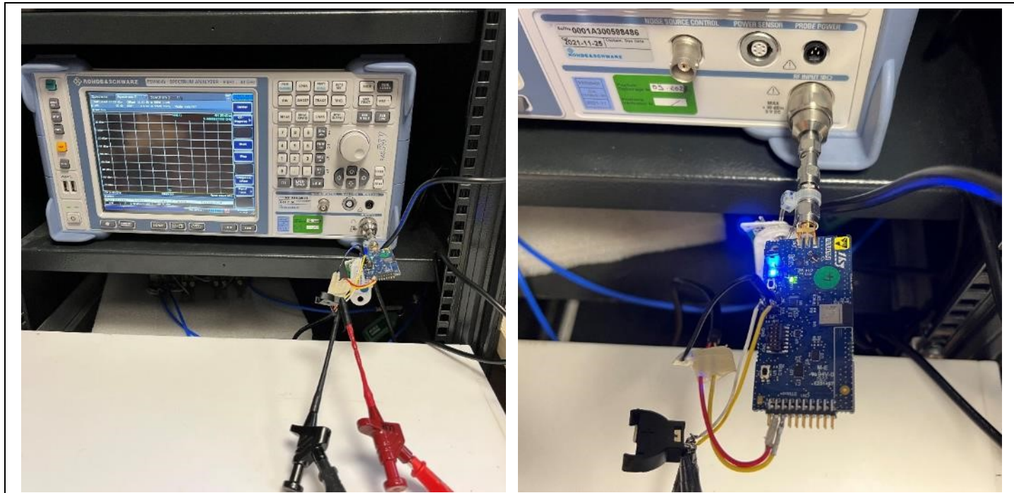
Photograph for Unwanted Emission into non-restricted frequency bands
