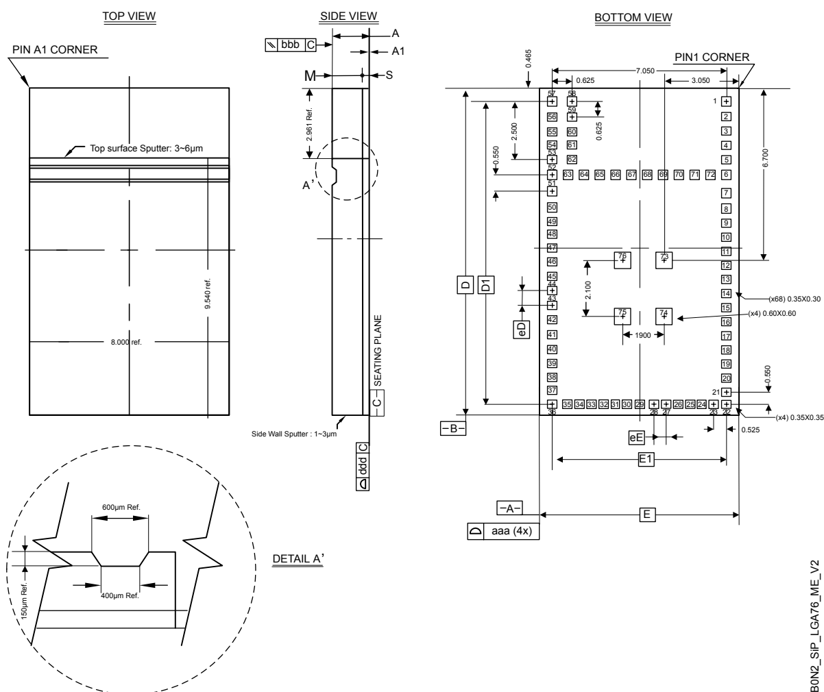
Figure 5. SiP-LGA76 - Outline
