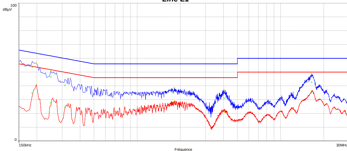
Line L1
