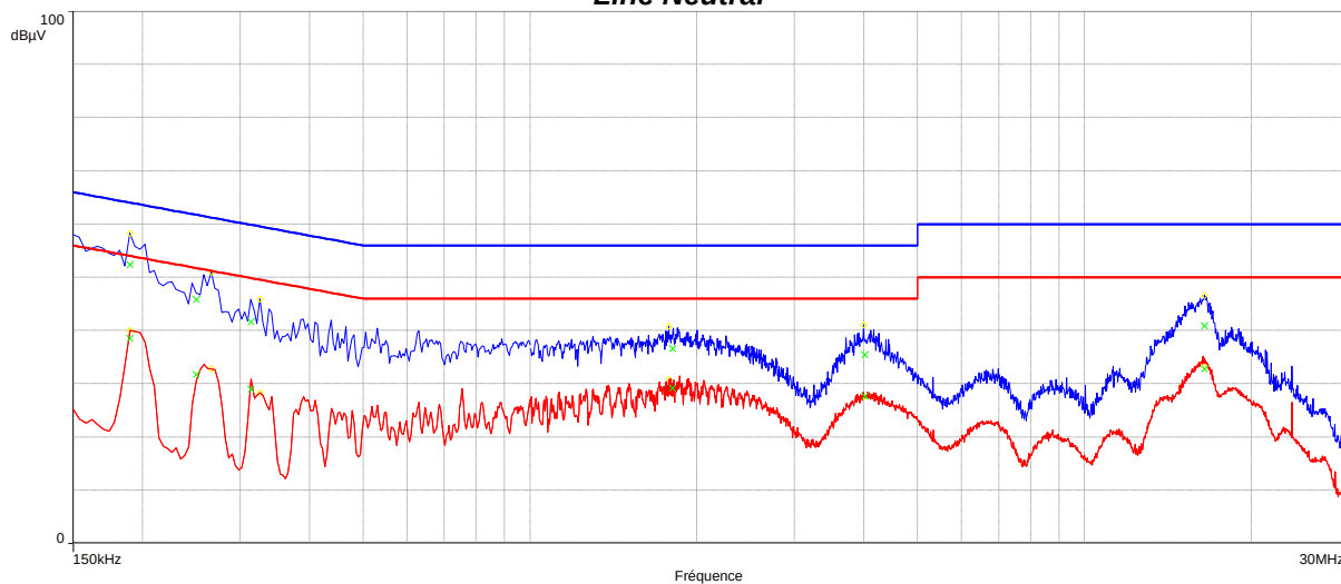
Line Neutral
