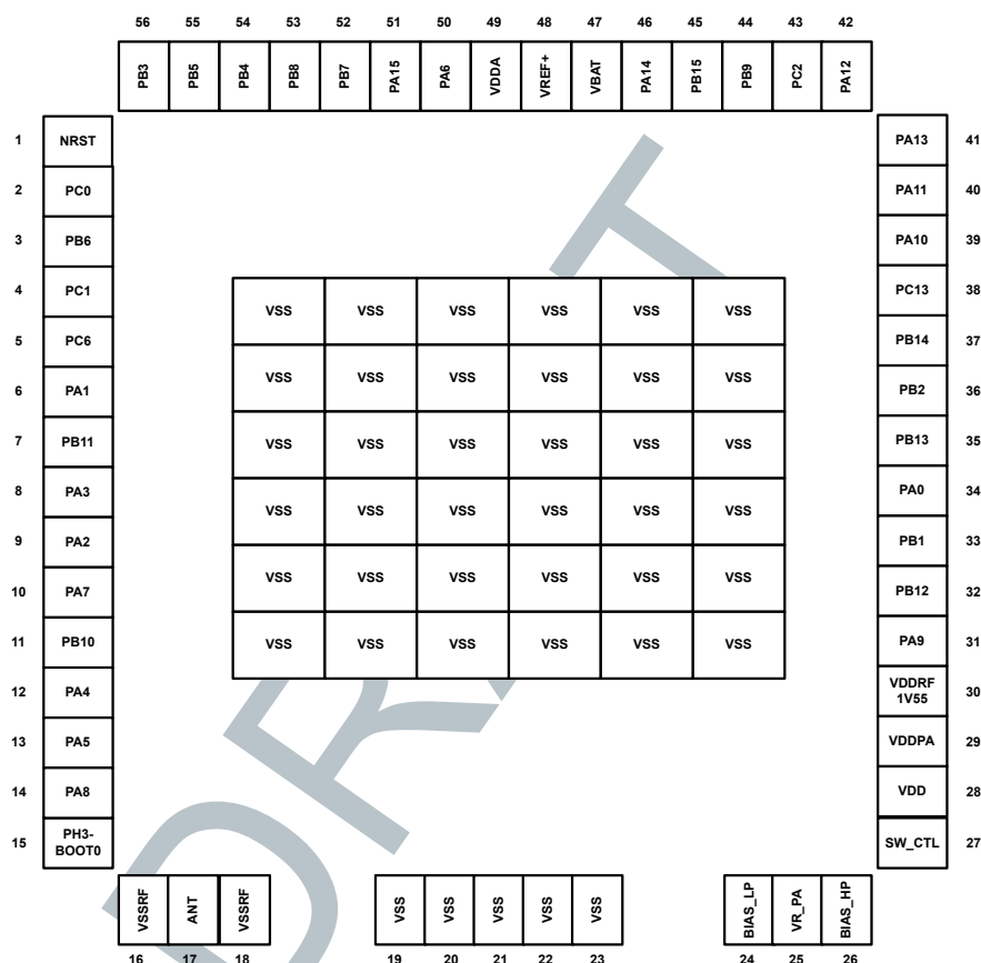
Figure 16. SIP LGA92 pinout
