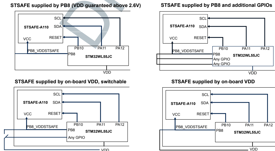
Figure 15. STSAFE configurations
