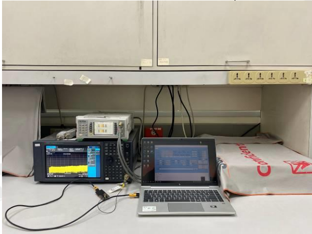
FCC_15_247_Thread_Conducted_Setup
