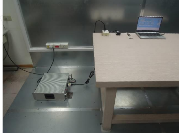
FCC_15_247_BT_Conduction_Setup
