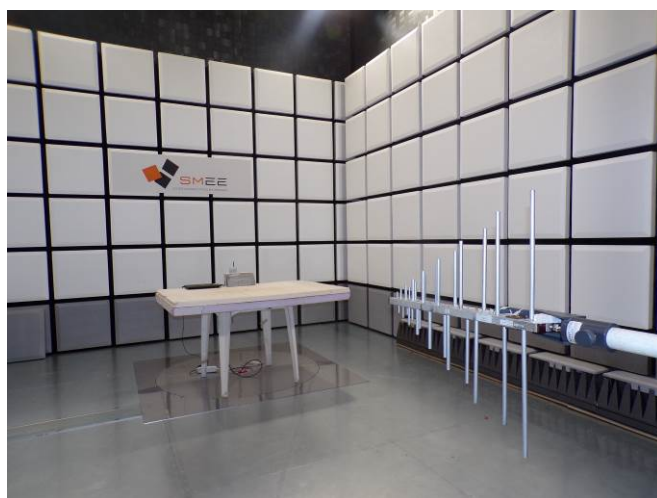
Test setup for frequency below 1GHz
