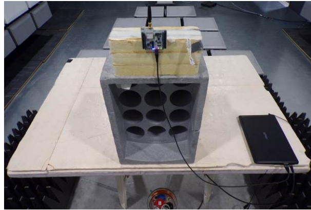
Test setup for frequency above 1GHz
