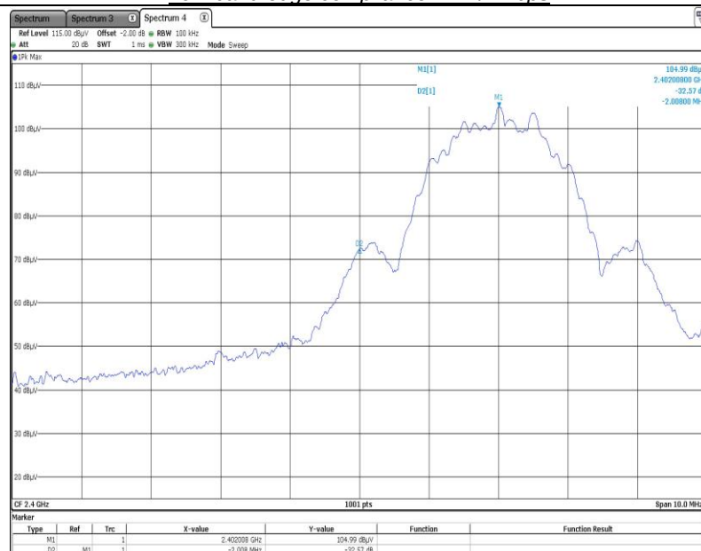
Low band edge compliance: BLE/2Mbps
