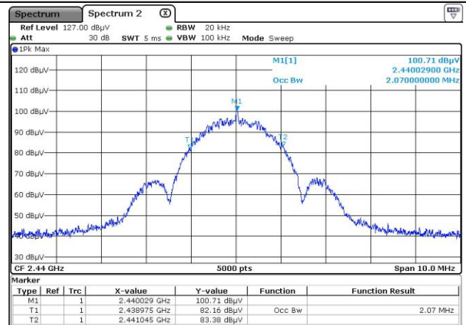
Mid channel
