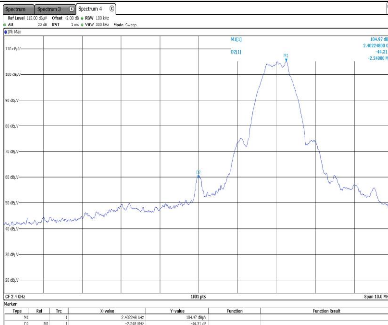
Low band edge compliance: BLE/1Mbps
