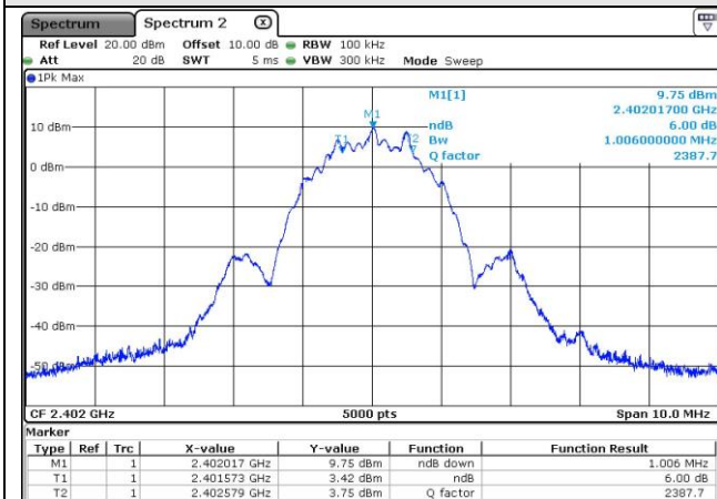
Low channel
