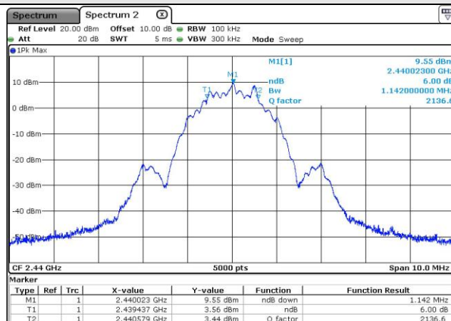
Mid channel
