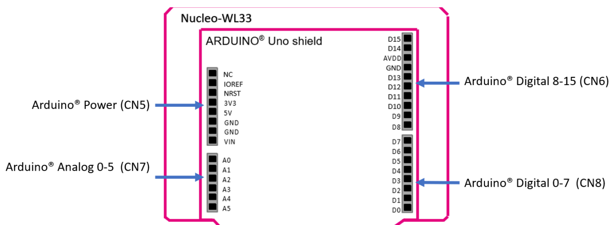
Figure 13 : ARDUINO® Uno connectors and shield location
