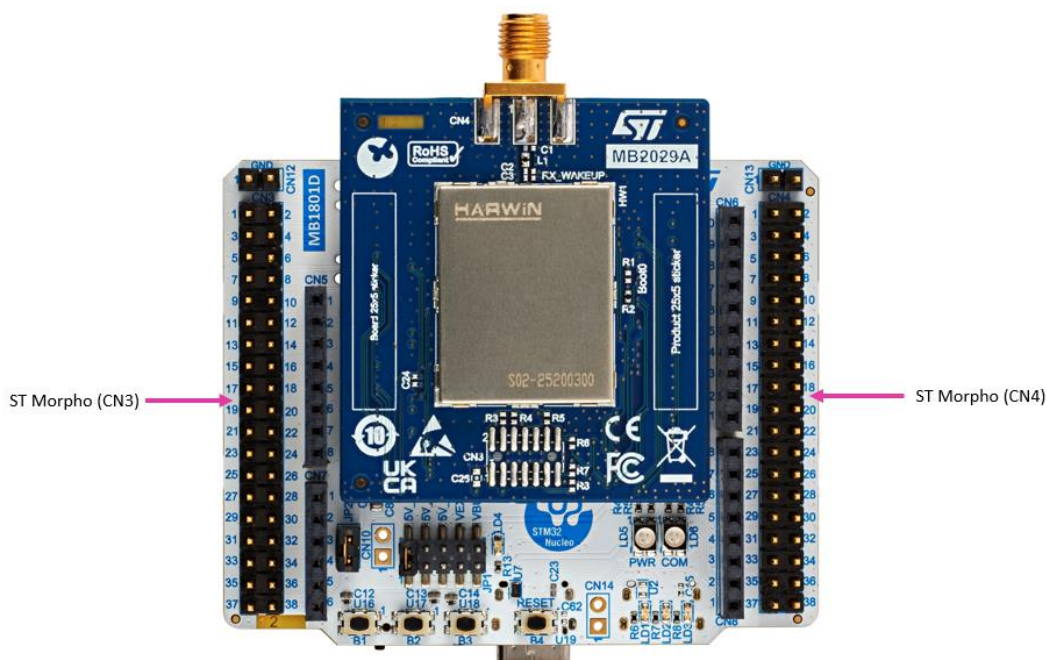
Figure 14 : ST morpho connectors location
