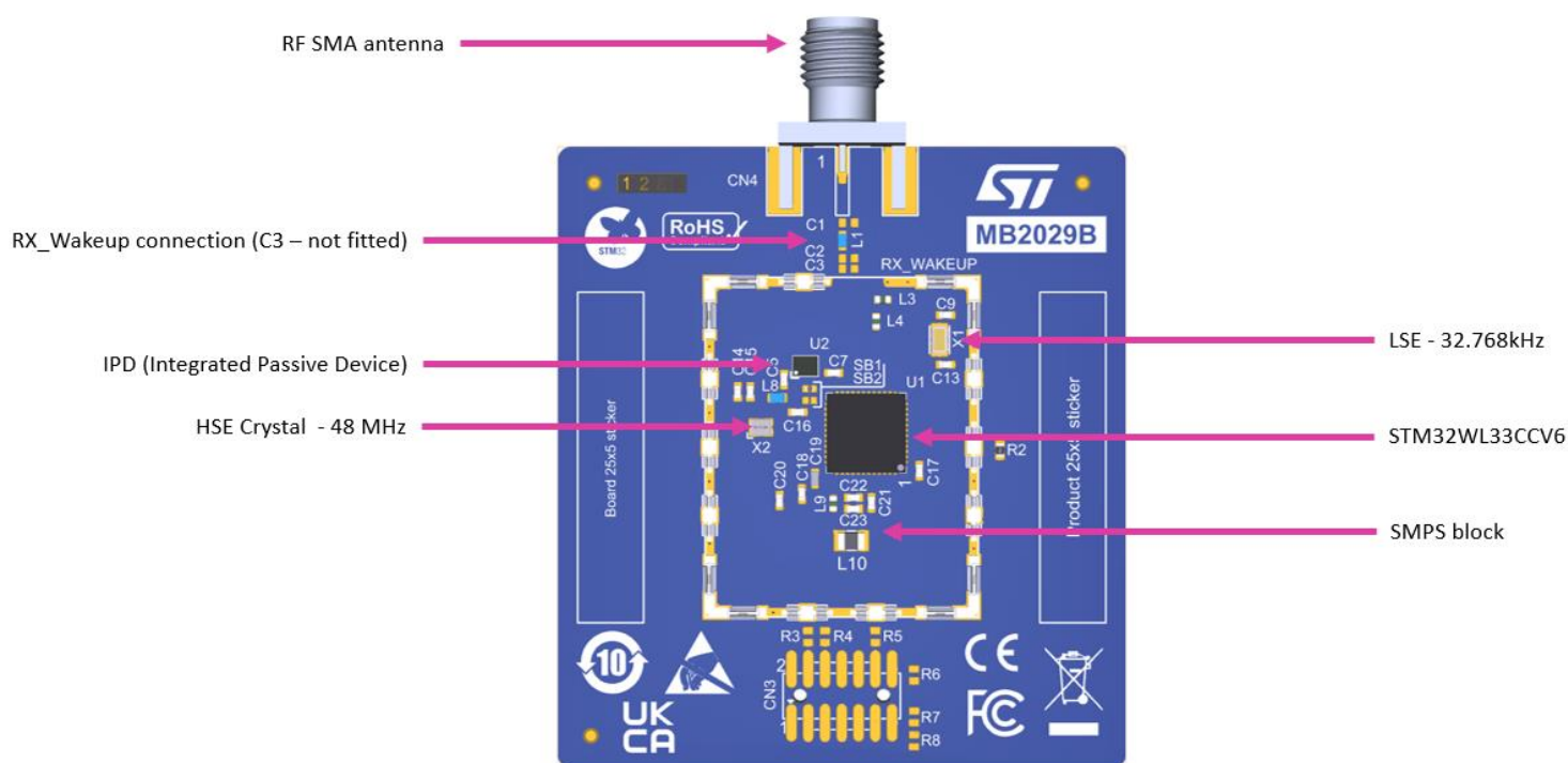
Figure 4 : NUCLEO-WL33CC PCB details of the MCU RF board MB2029
