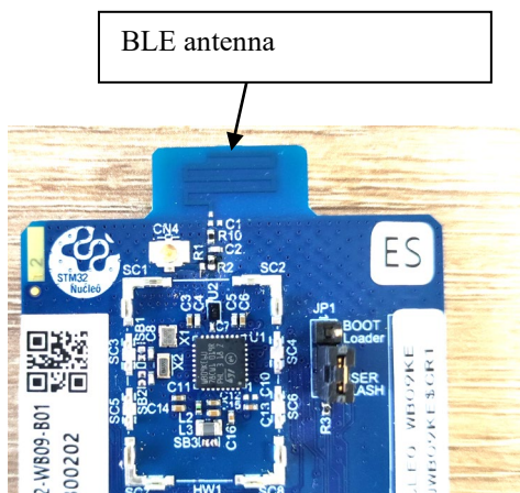
Cover removed (RF part)
