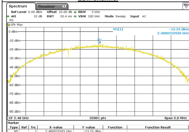
High channel
