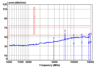
2.4G_SRD_TX_MID_Horizontal
