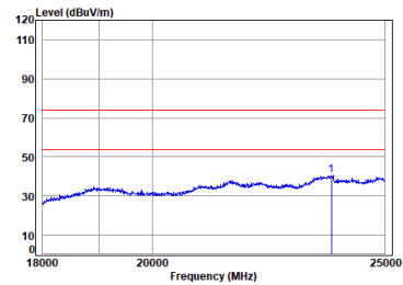
2.4G_SRD_TX_MID_Vertical
