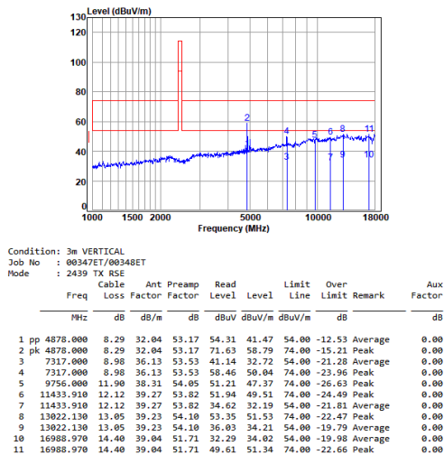
2.4G_SRD_MID_TX_Vertical
