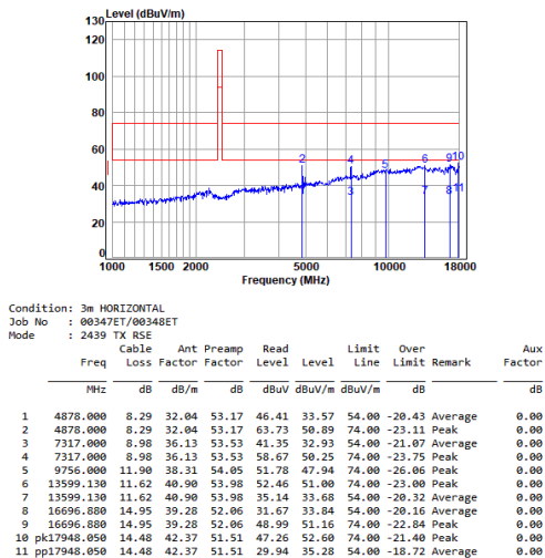
2.4G_SRD_MID_TX_Horizontal
