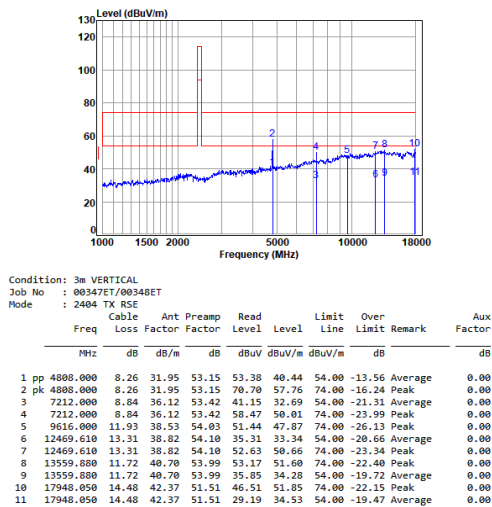
2.4G_SRD_LOW_TX_Vertical
