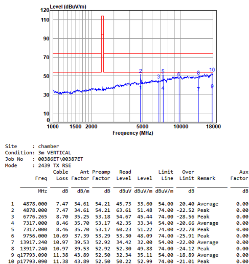
MIN-1052 2.4G SRD_TX_CH_M_Vertical
