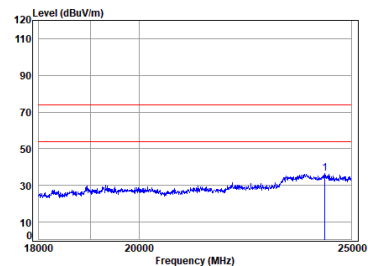
MIN-1052 2.4G SRD_TX_CH_M_Vertical
