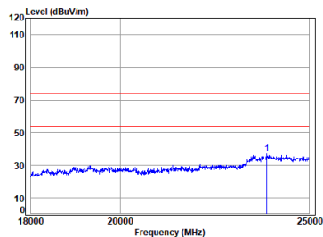
MIN-1052 2.4G SRD_TX_CH_M_Horizontal
