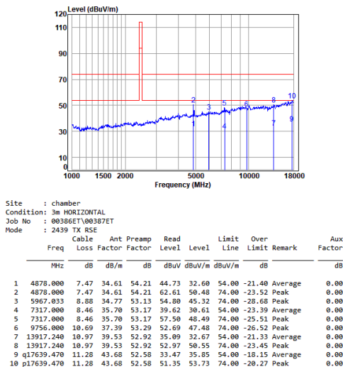
MIN-1052 2.4G SRD_TX_CH_M_Horizontal
