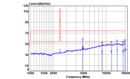
2.4G_SRD_TX_MID_Horizontal
